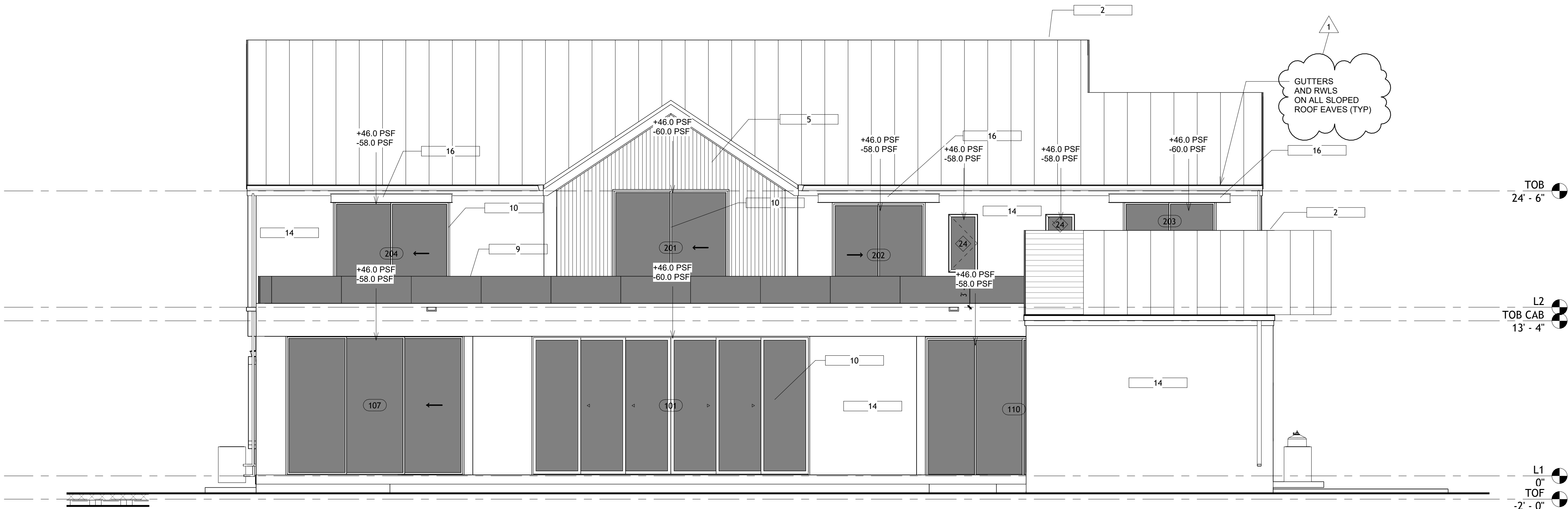
1 North Architectural Building Elevation 3/16" = 1'-0"
