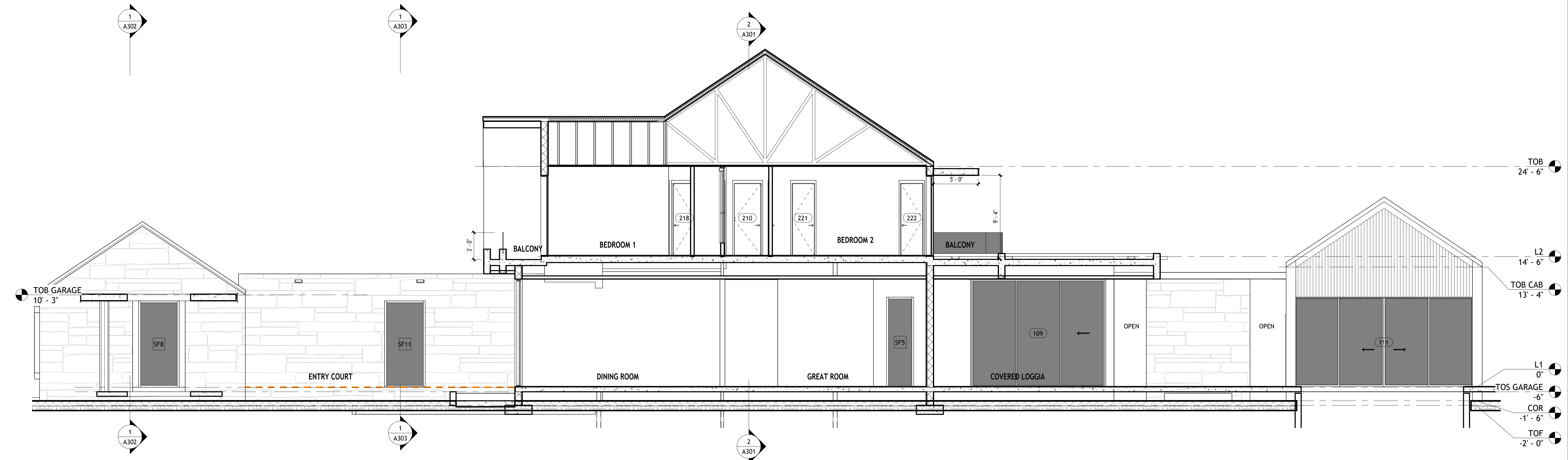
2 Section 1 3/16" = 1'-0"
