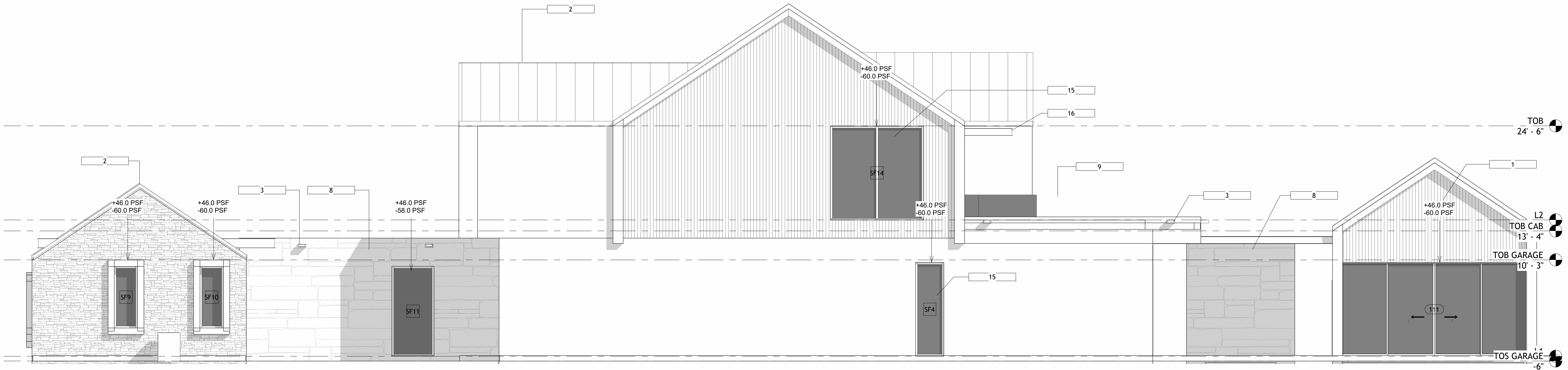
1 South Architectural Building Elevation 3/16" = 1'-0"
