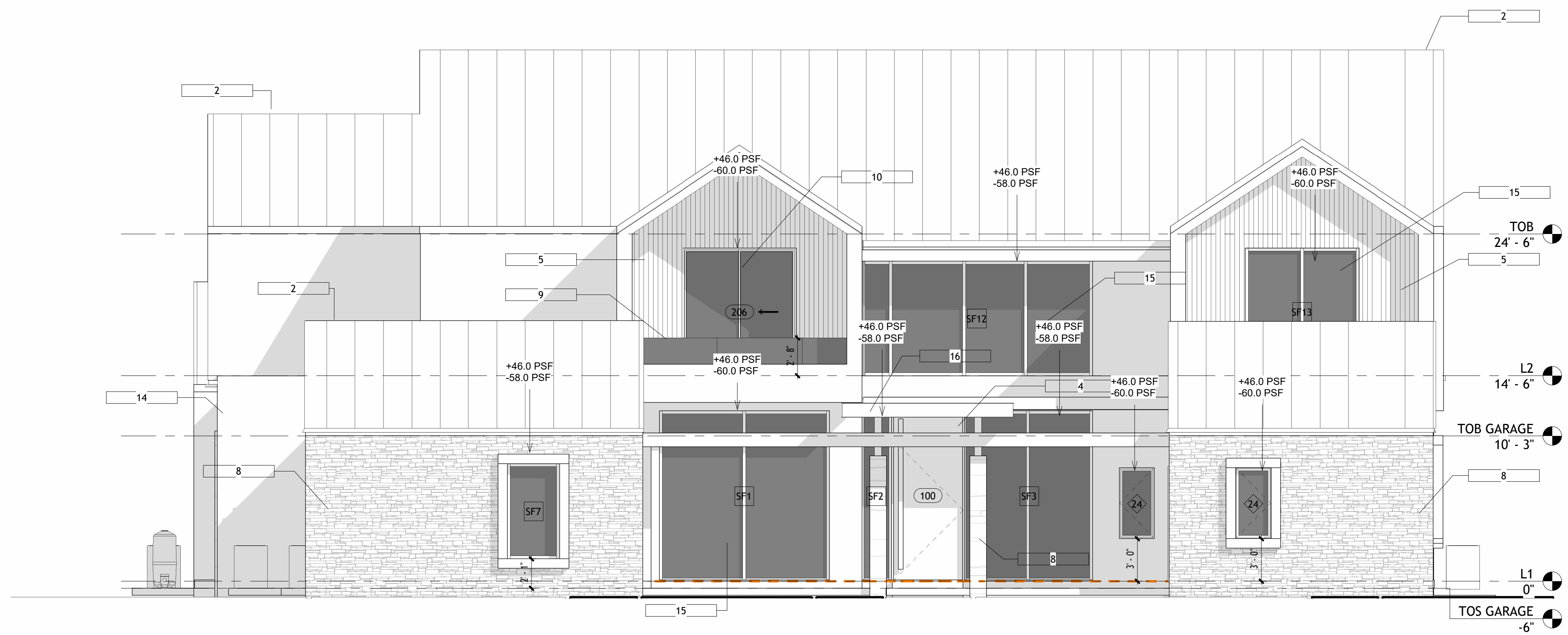
2 West Architectural Building Elevation 3/16" = 1'-0"
