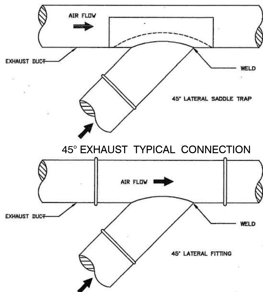
NOTE: COMPLY WITH FIGURE 3-4 OF LATEST HVAC DUCT CONSTRUCTION STANDARDS METAL AND FLEXIBLE TYPICAL 45° LATERAL CONNECTION DETAIL N.T.S. KJTP-45
