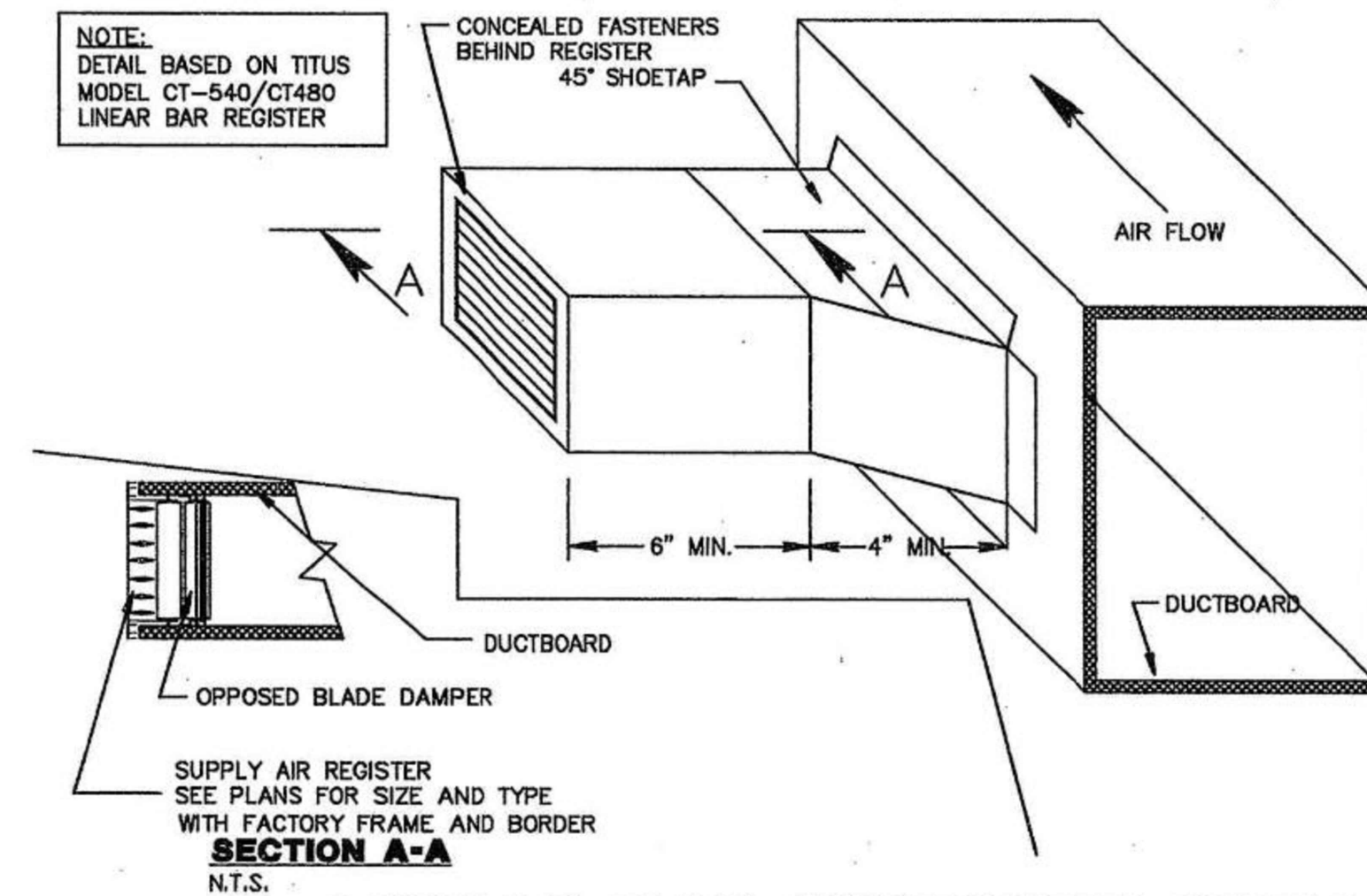
LINEAR BAR REGISTER DETAIL
