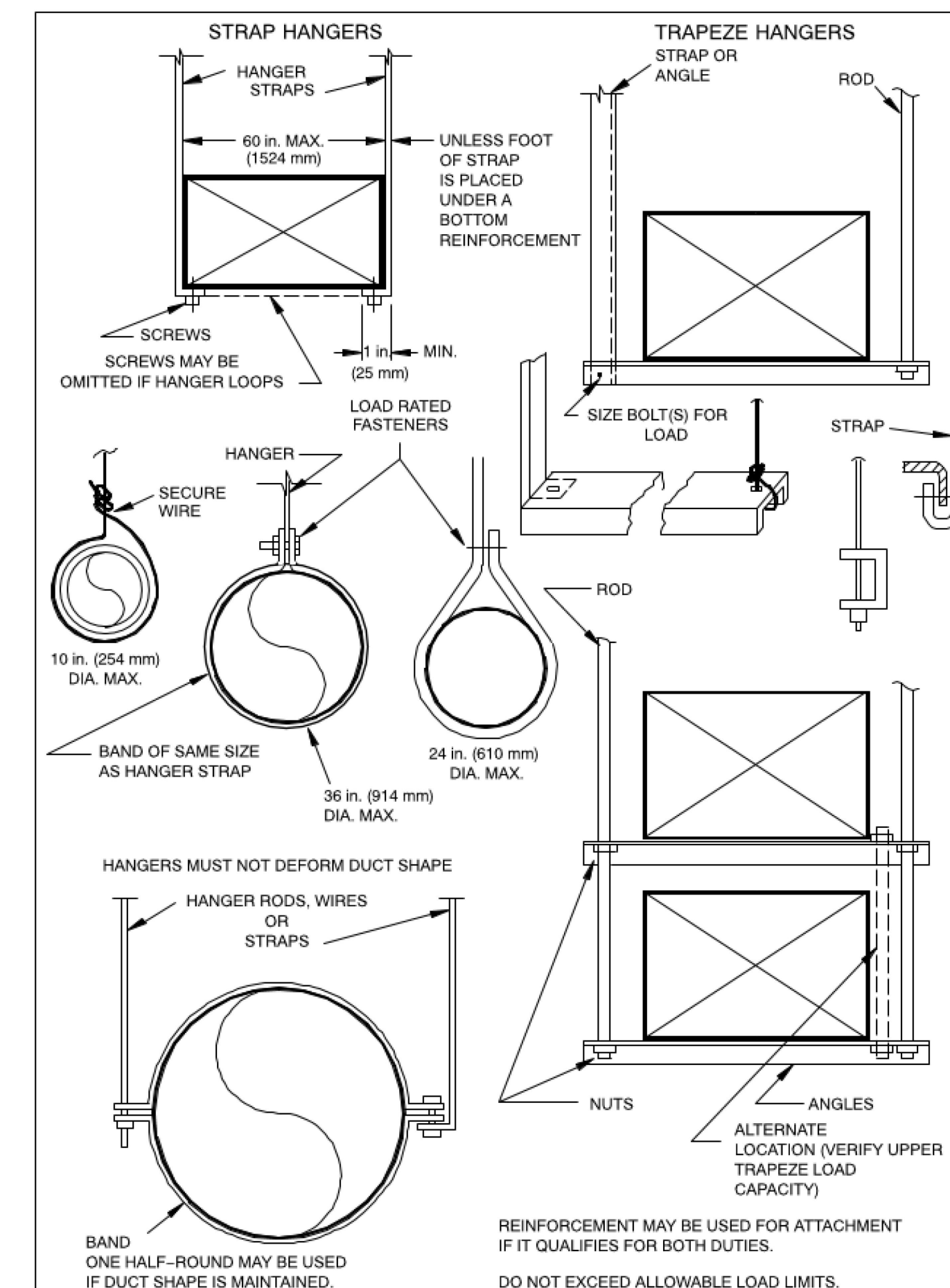
FIGURE 5-5 LOWER HANGER ATTACHMENTS
