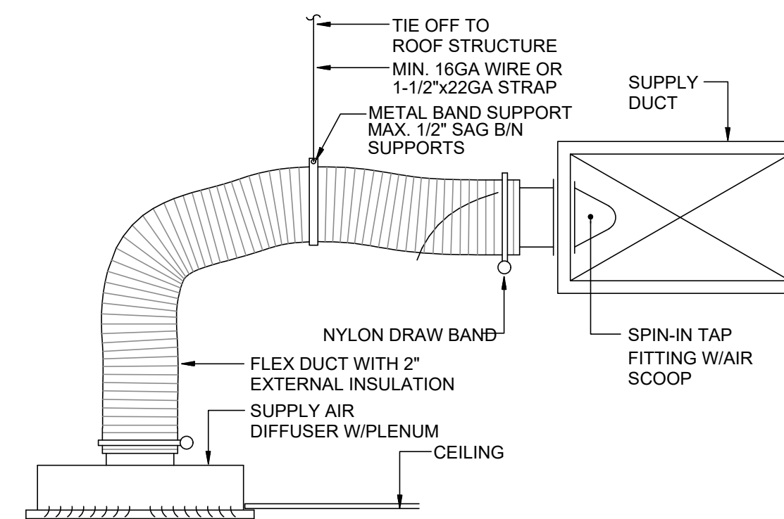
SUPPLY AIR DIFFUSER DETAIL
