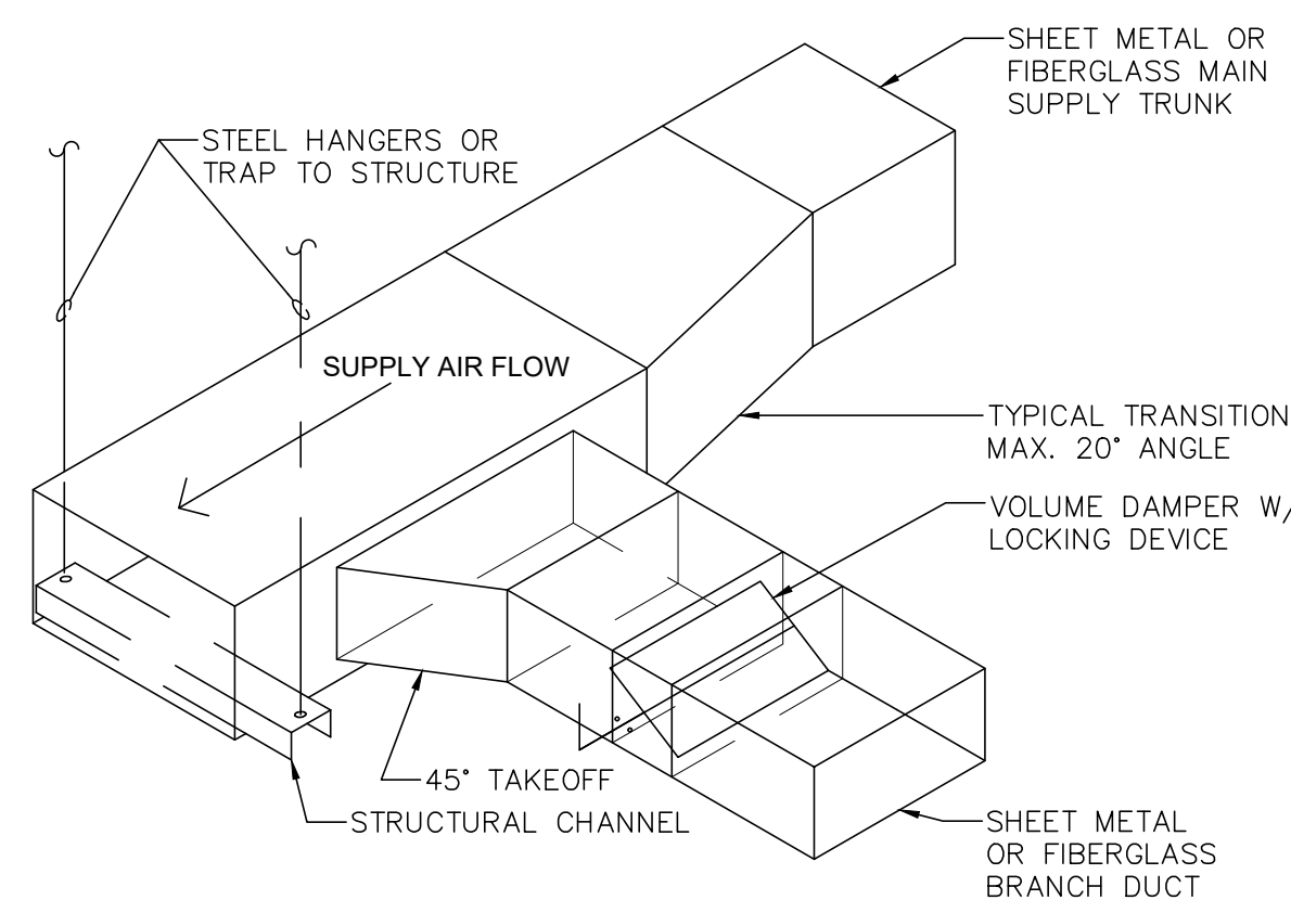
BRANCH DUCT TAKEOFF DETAIL NTS.
