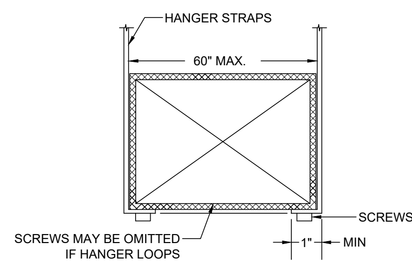
DUCT HANGER DETAIL
