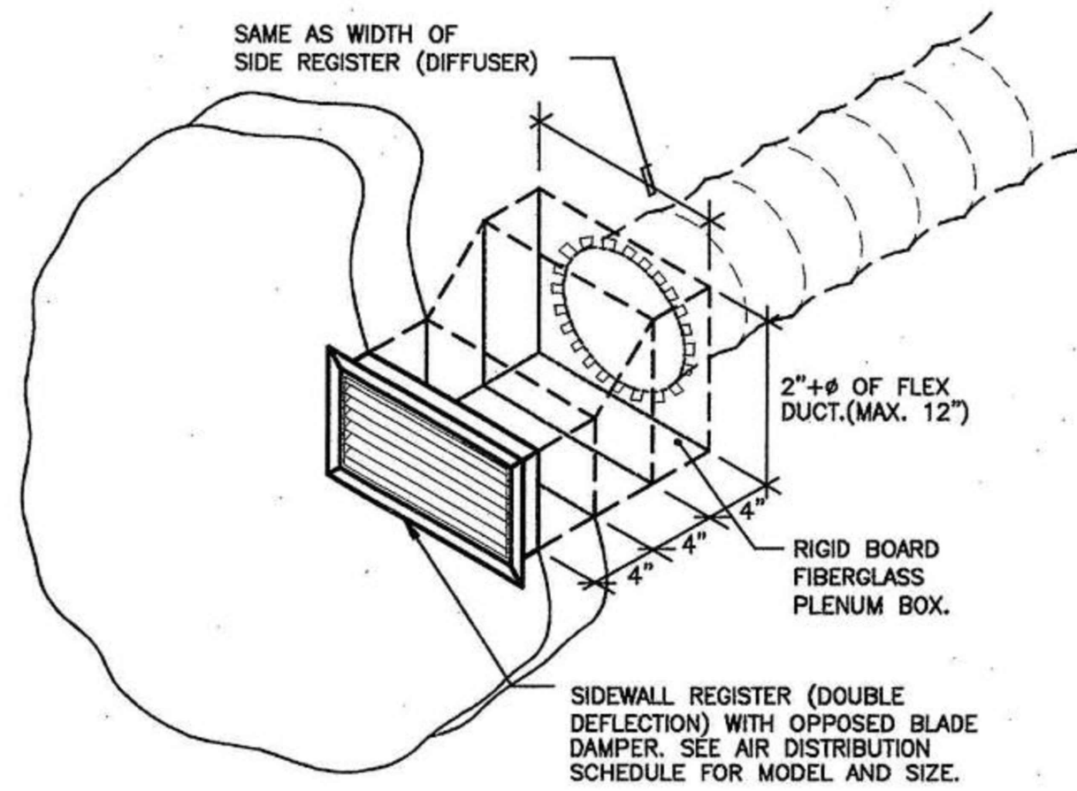
SIDEWALL REGISTER DETAIL
