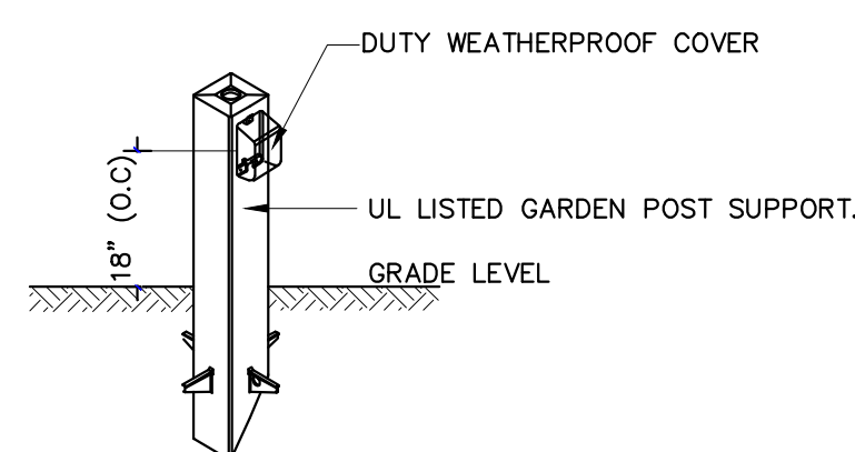
G.F.C.I. RECEPTACLE MOUNTING DETAIL
