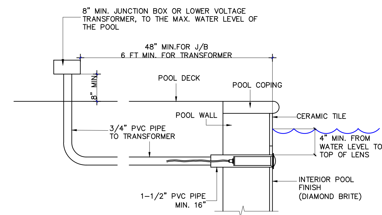
NICHELESS LIGHT DETAIL NO SCALE
