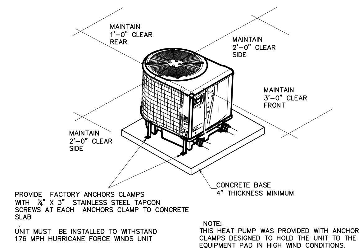
HEAT PUMP MOUNTING DETAIL
