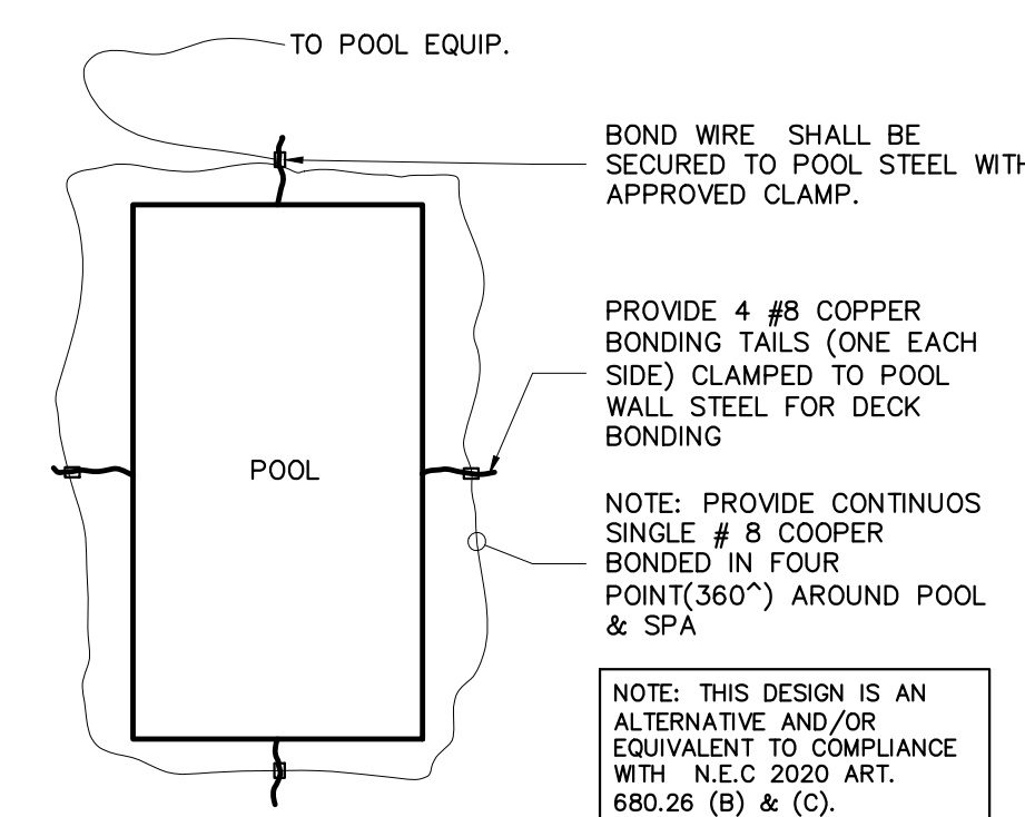
POOL BOND SCHEMATIC
