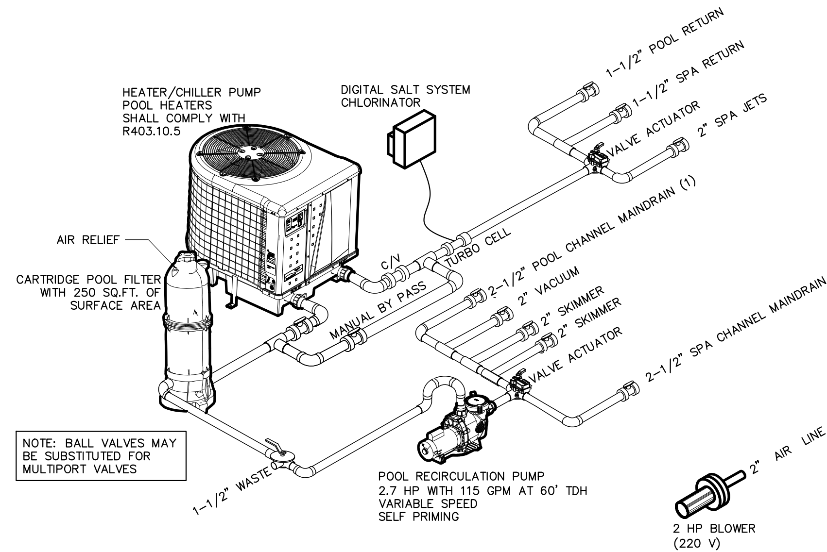
POOL ISOMETRIC
