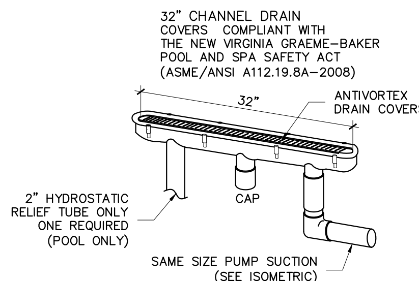
CHANNEL MAINDRAIN DETAIL (SPA)
