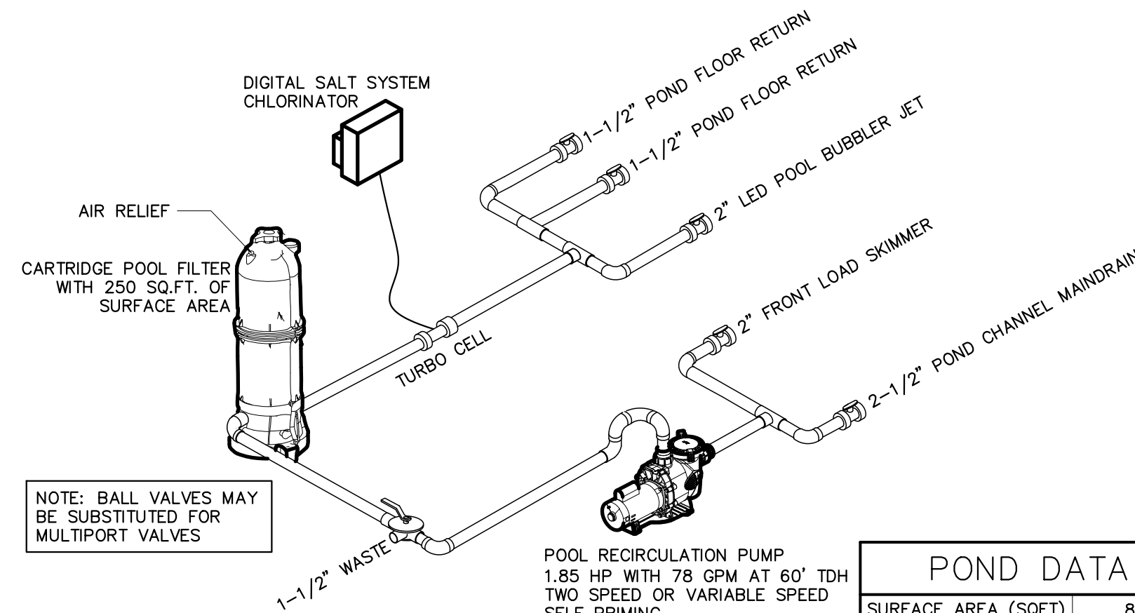
POND ISOMETRIC
