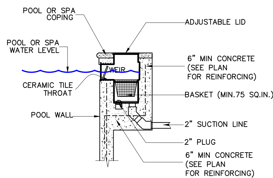
SKIMMER DETAIL
