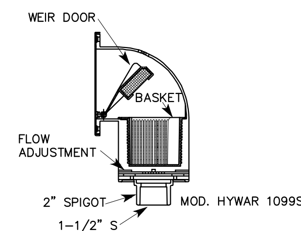
FRONT LOAD SKIMMER DETAIL
