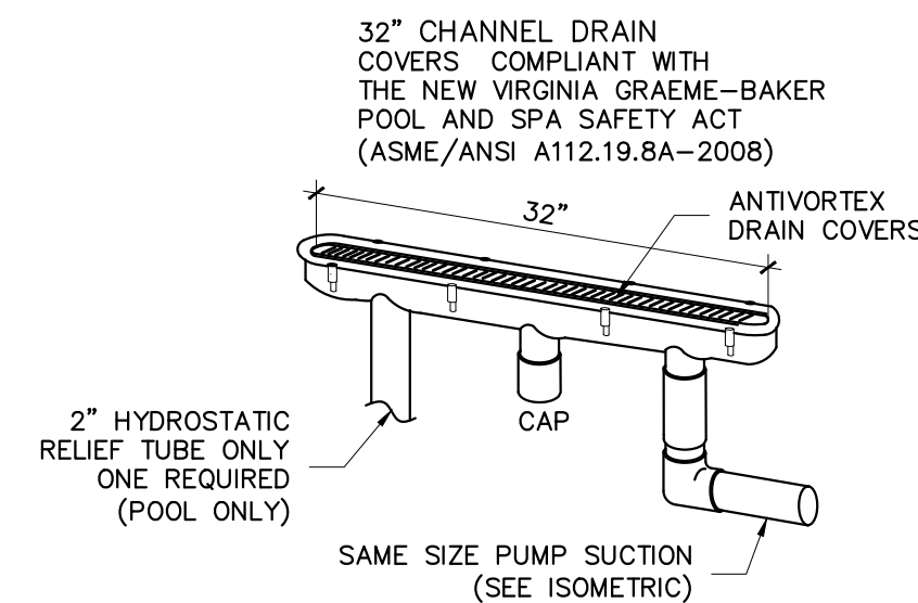
CHANNEL MAINDRAIN DETAIL (POND)
