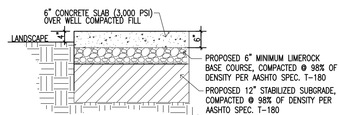
DRIVEWAY TYPICAL SECTION
