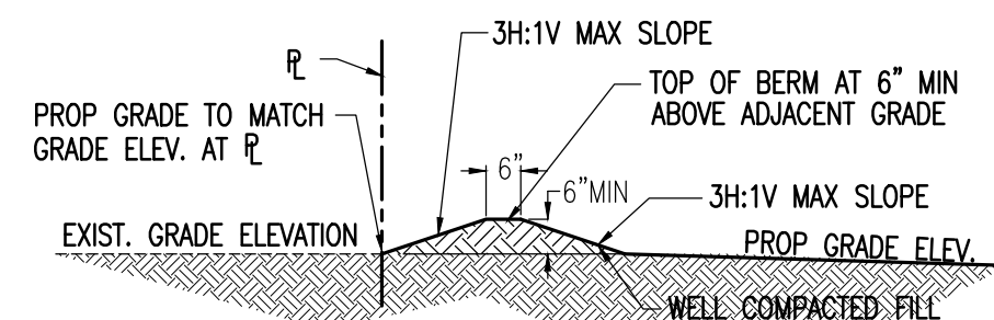
BERM DETAIL
