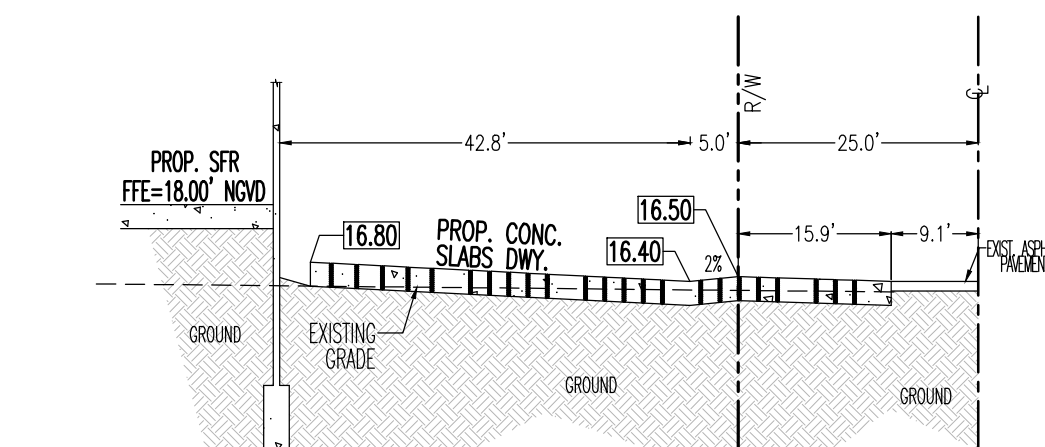
SECTION C
