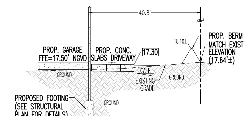
SECTION F
