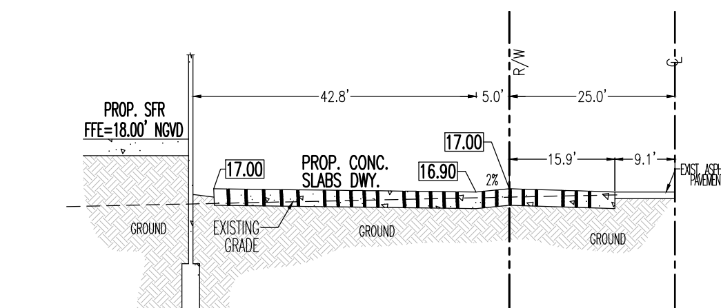
SECTION B
