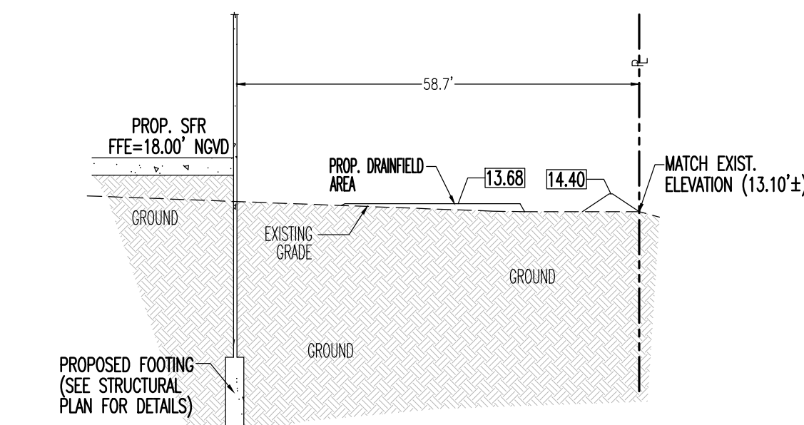
SECTION D
