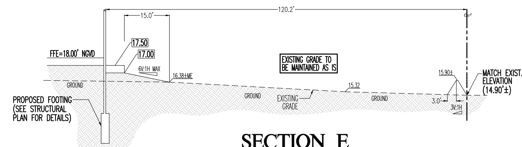
SECTION E
