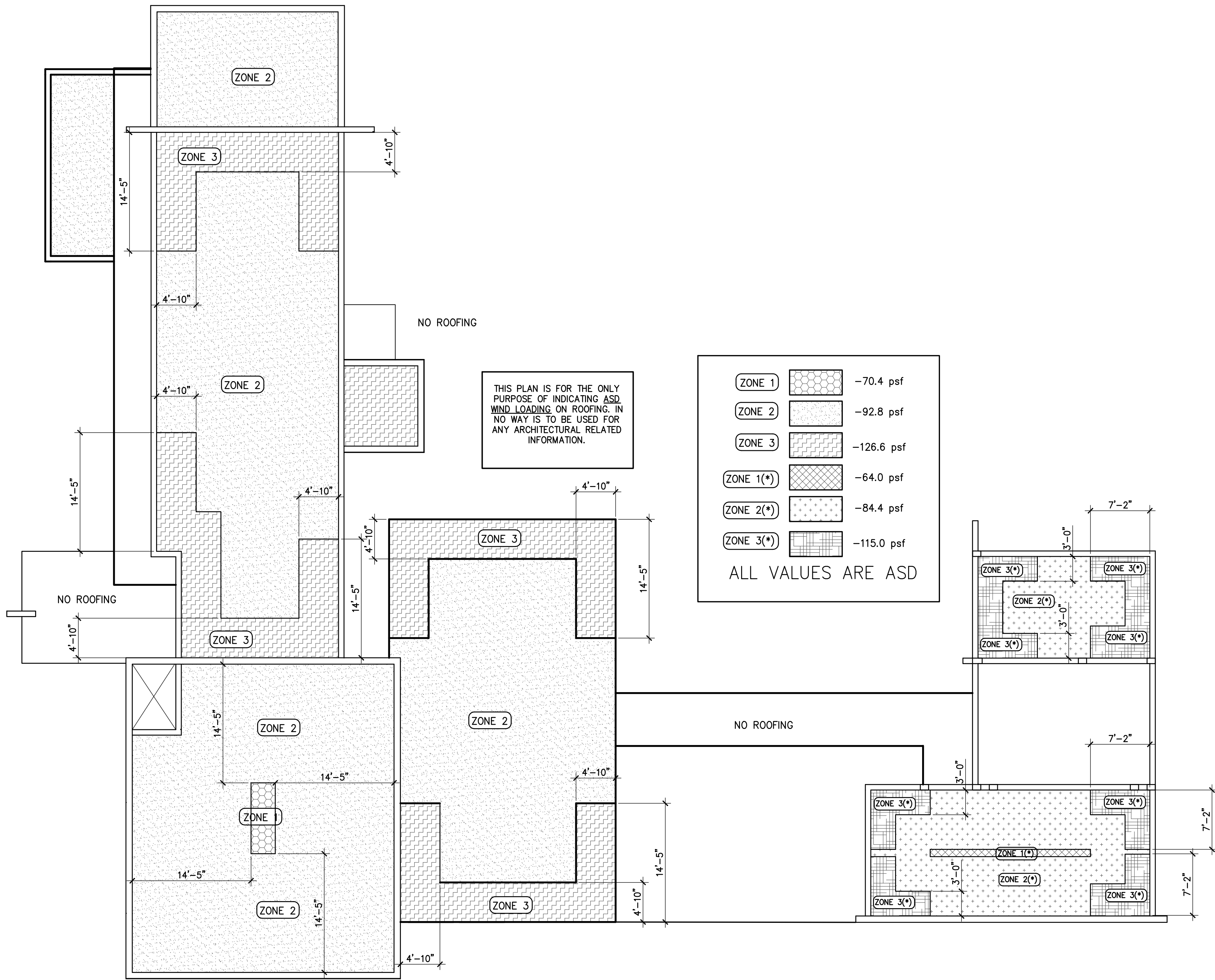
ROOF WIND UPLIFT
