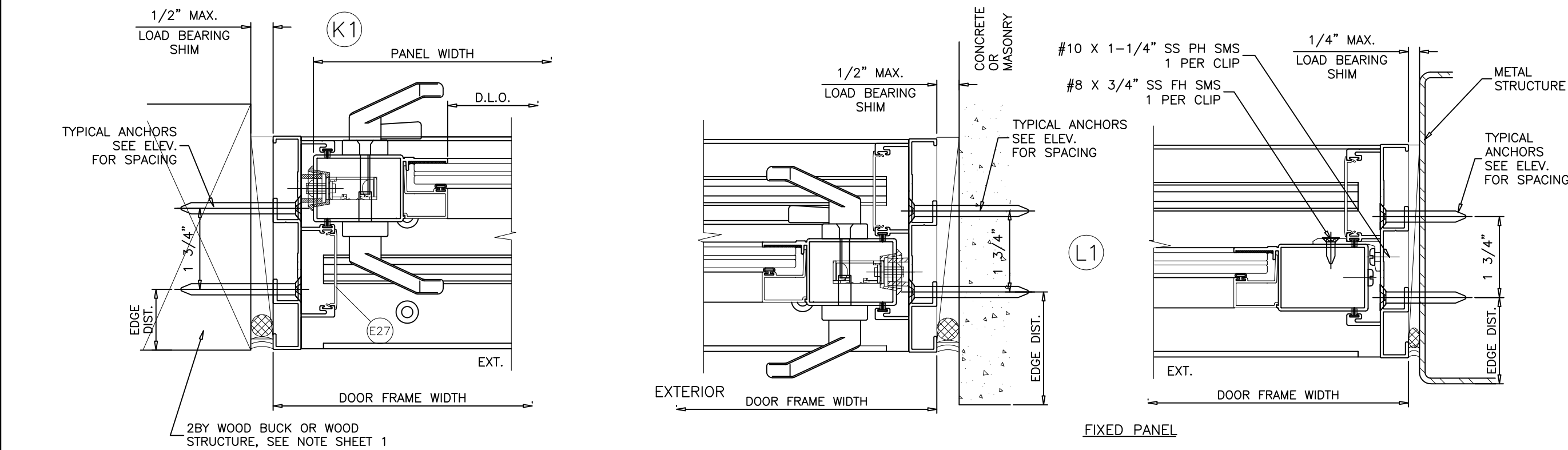
2 TRACK DOOR HORIZONTAL DETAILS
