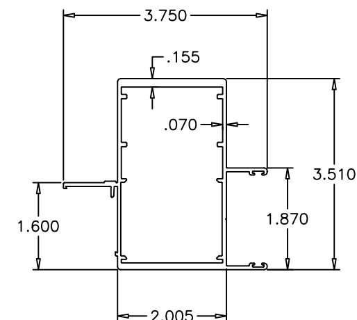
E14 OUTER TRACK ASTRAGAL STILE
