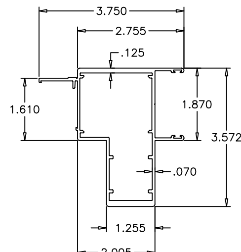
E9 INTERIOR TRACK ASTRAGAL STILE
