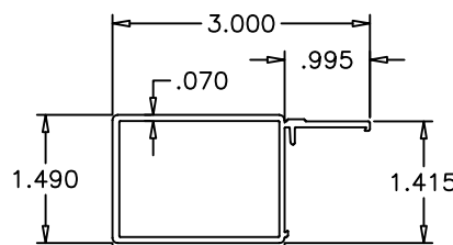
E6 MAIN STILE
