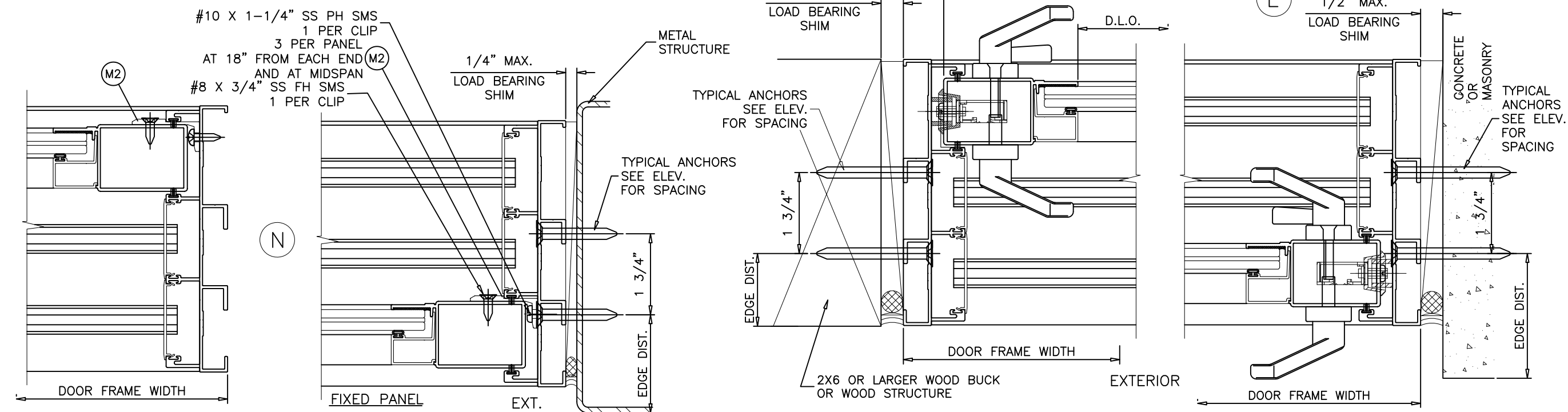
3 TRACK DOOR HORIZONTAL DETAILS
