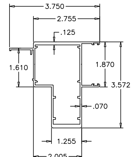
E22 INTERIOR TRACK ASTRAGAL (OPTIONAL)
