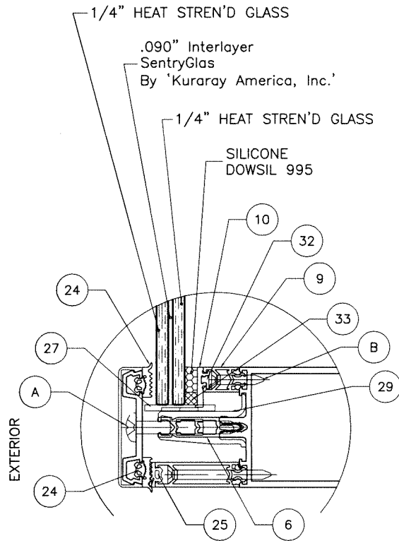
GLASS TYPE 'A' 9/16" OVERALL NOMINAL THK.
