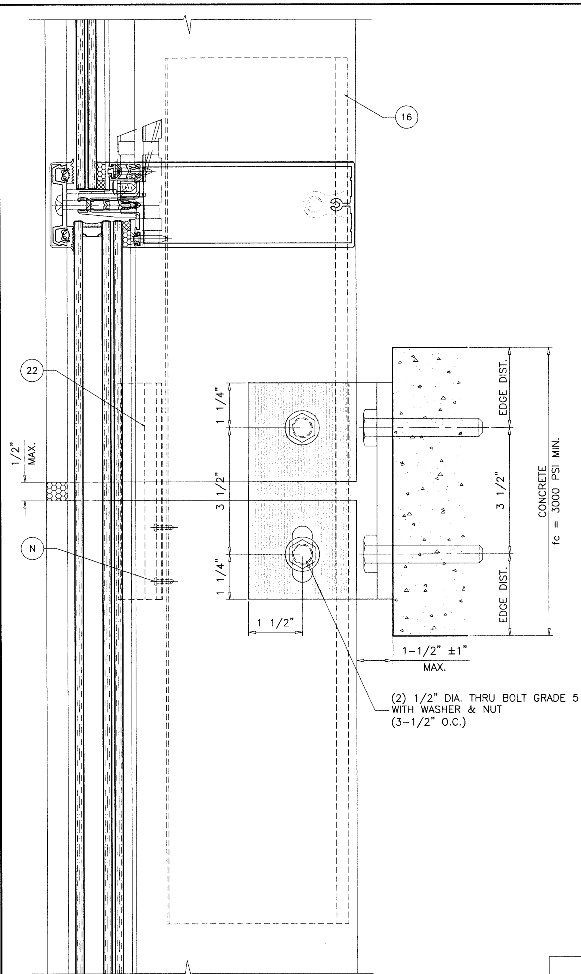
INTERMEDIATE ANCHORS
