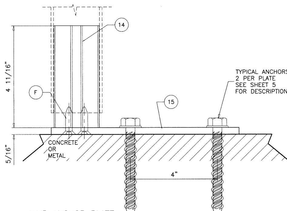
JAMB ANCHOR PLATE AT HEAD/SILL
