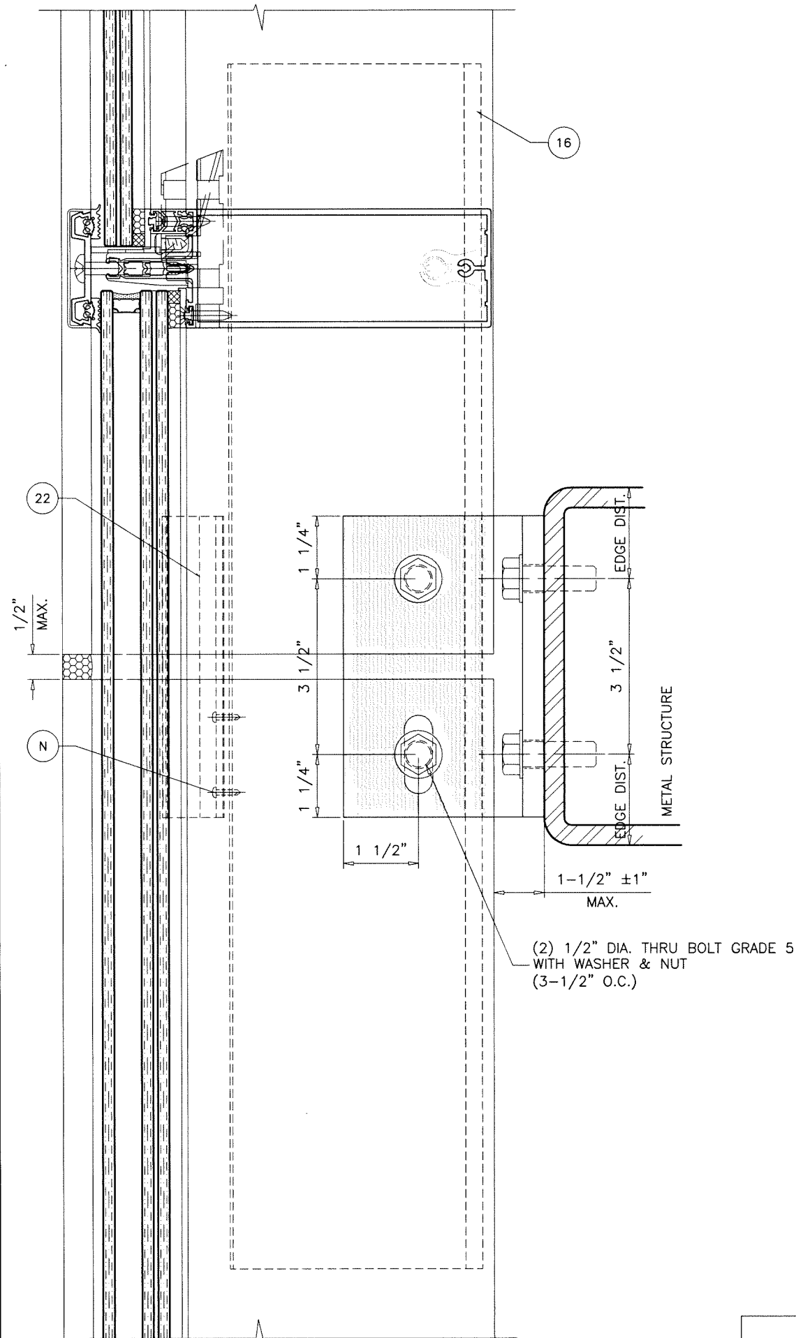
INTERMEDIATE ANCHORS
