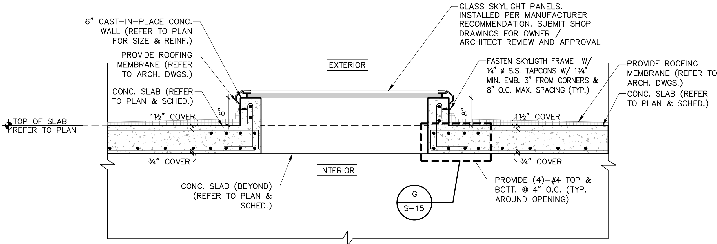
SKYLIGHT CURB DETAIL B SCALE : 3/4" = 1'-0"
