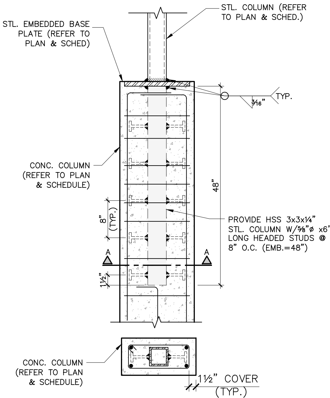
STL. COLUMN DETAIL C SCALE : 3/4"=1'-0"
