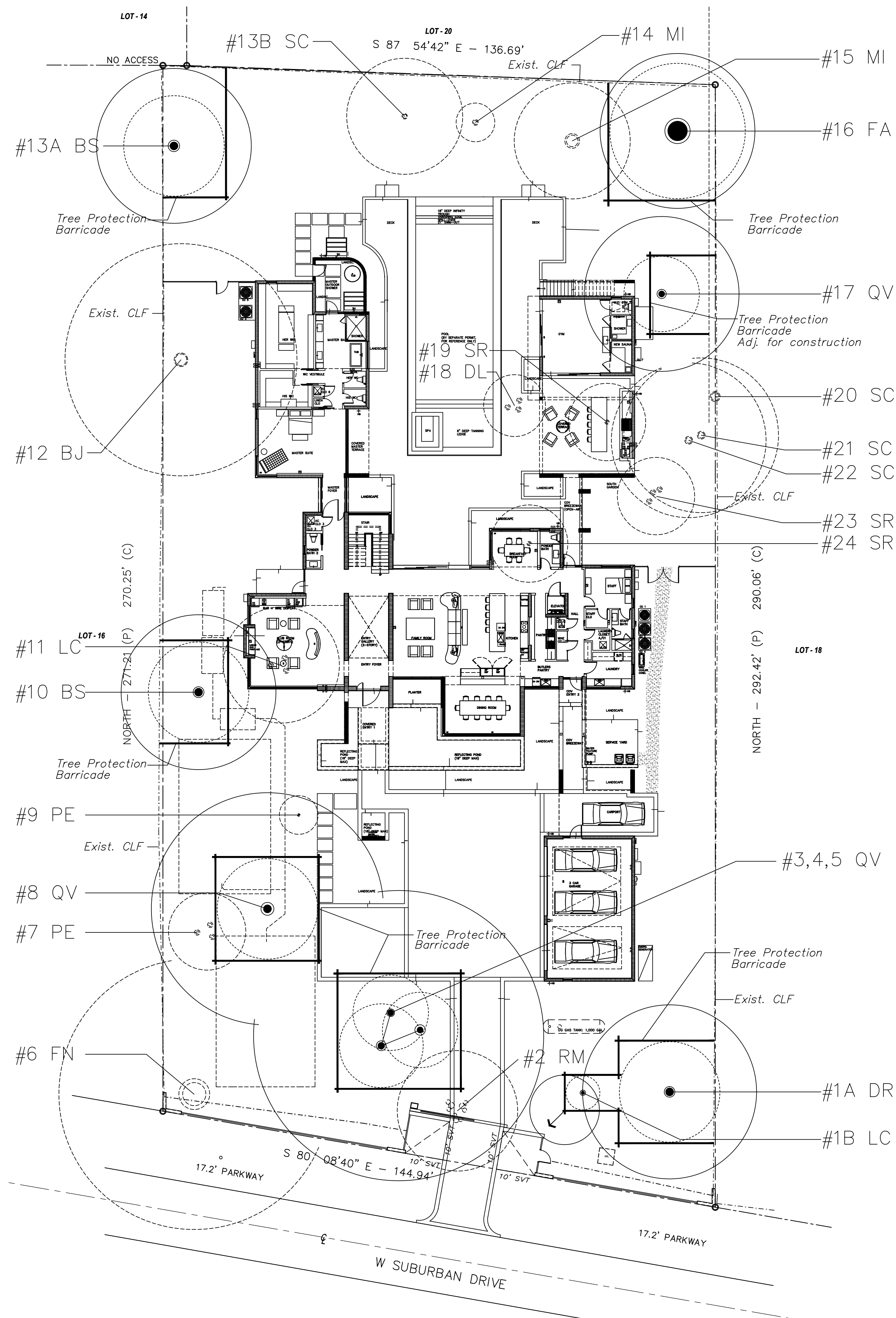
TREE SURVEY / DISPOSITION PLAN SCALE: 1/16" = 1'-0"
