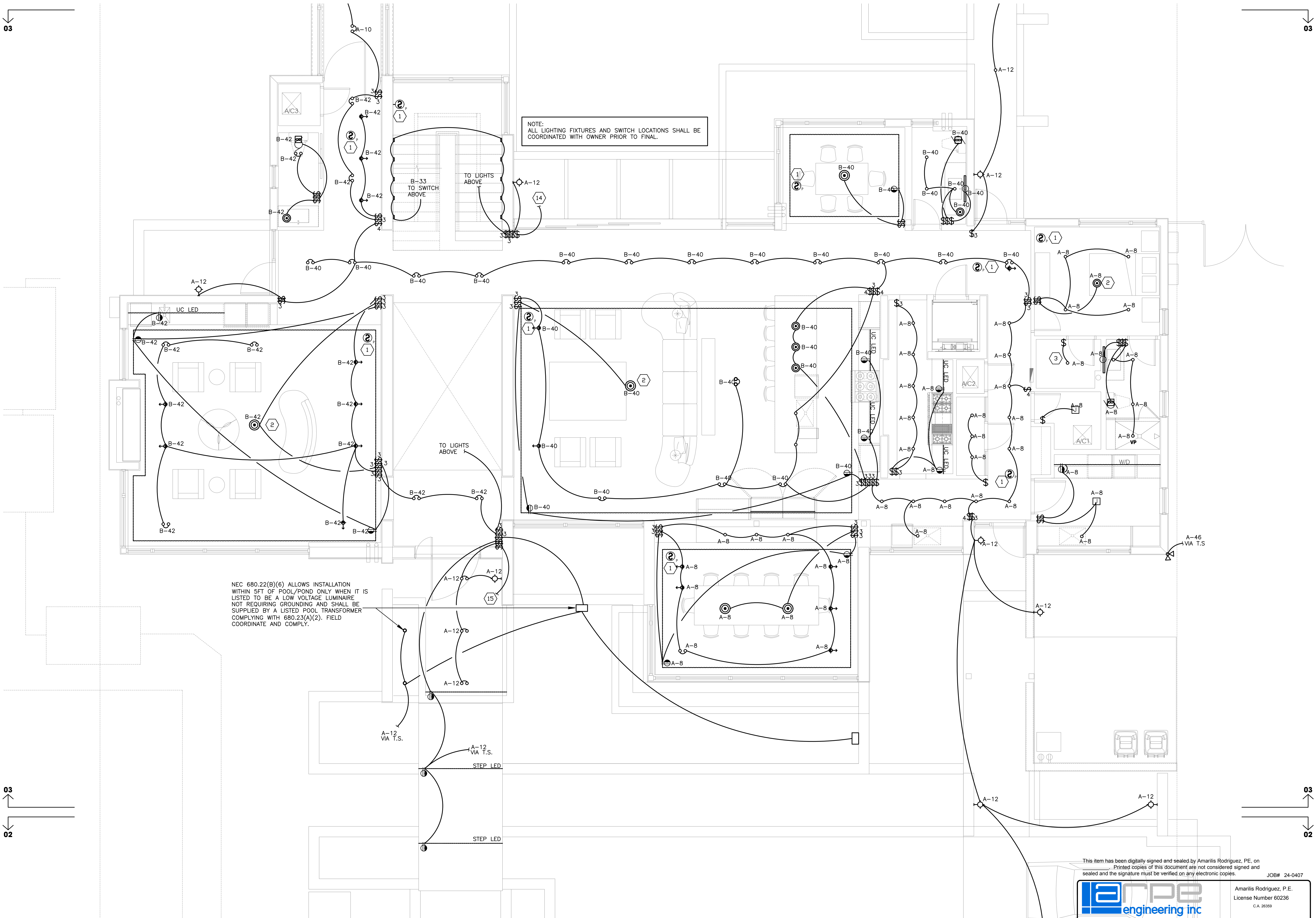
LIGHTING PARTIAL FIRST RCP: 03 SCALE: 1/4" = 1'-0"
