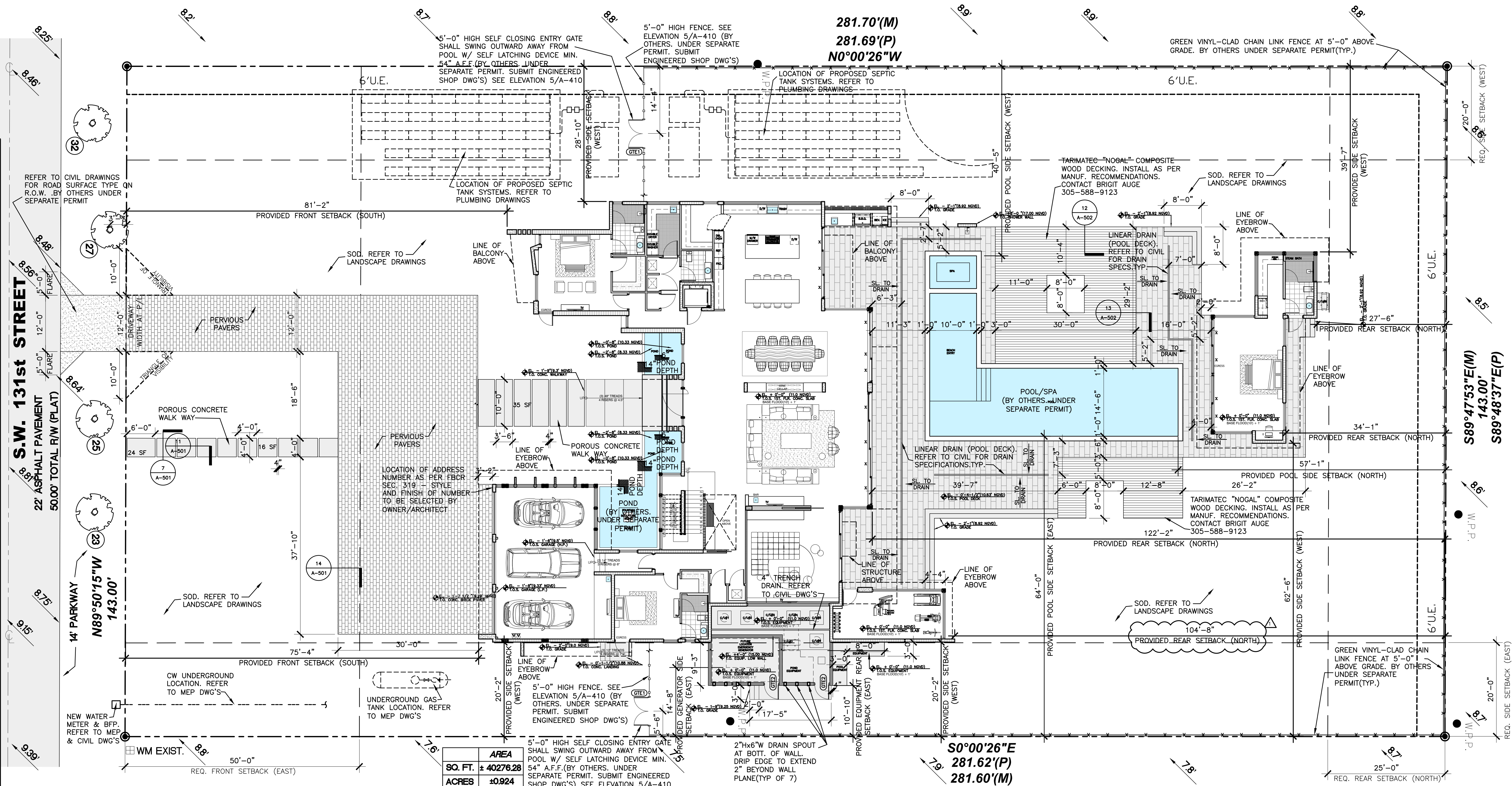
SITE PLAN SCALE: 3/32"=1'-0"
