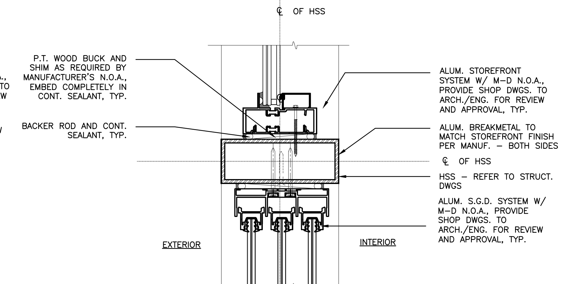
4 A-504 STOREFRONT/SLIDING GLS DOOR-JAMB DETAIL SCALE: 3"=1'-0"
