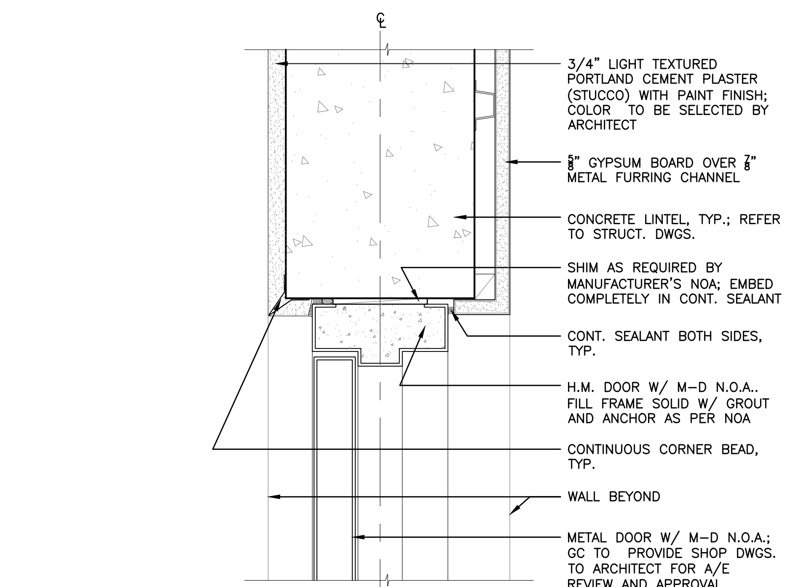
15 A-504 H.M. DOOR HEAD DETAIL SCALE: 3"=1'-0"
