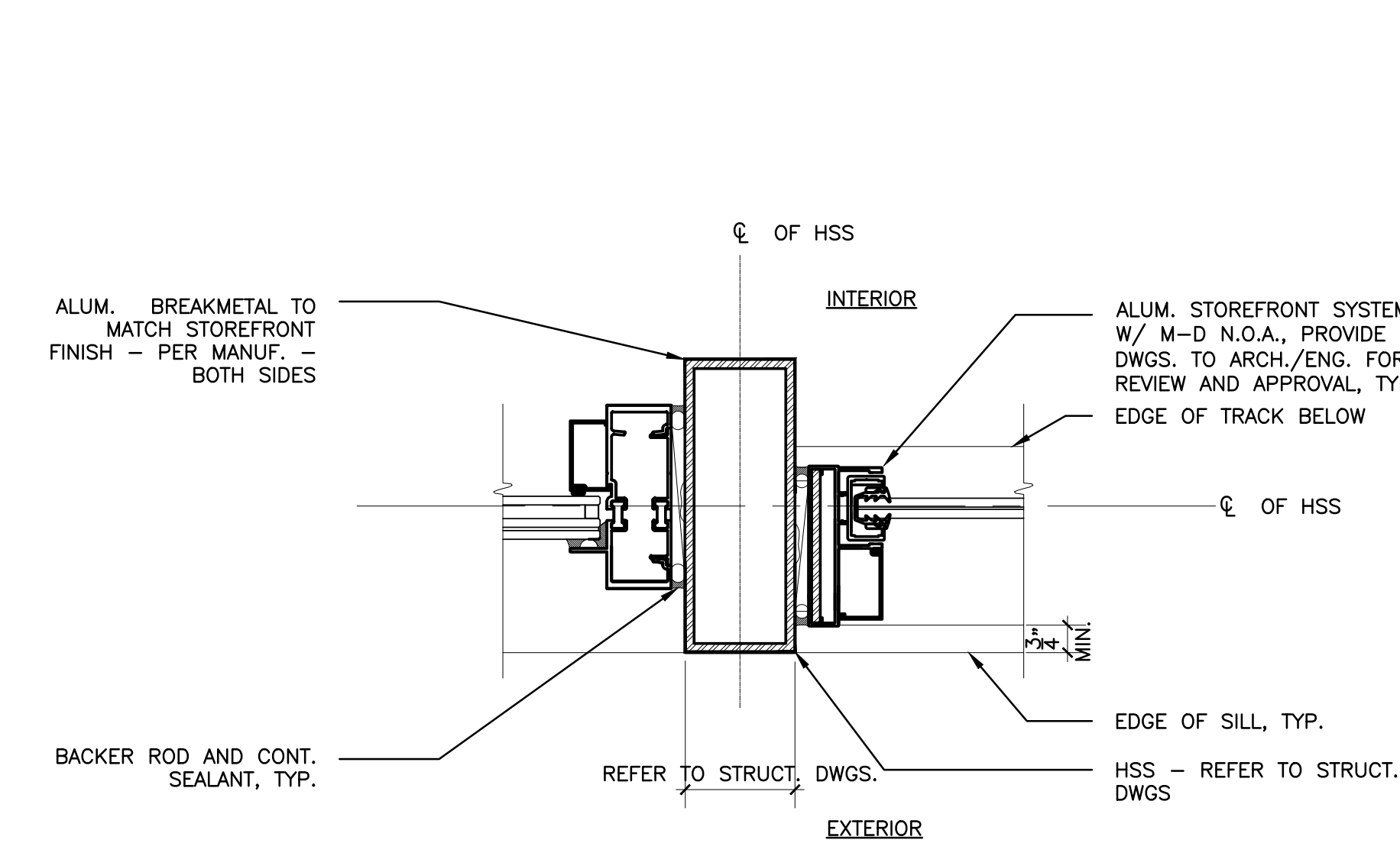
11 A-504 STOREFRONT/SLIDING GLS DOOR-JAMB DETAIL SCALE: 3"=1'-0"
