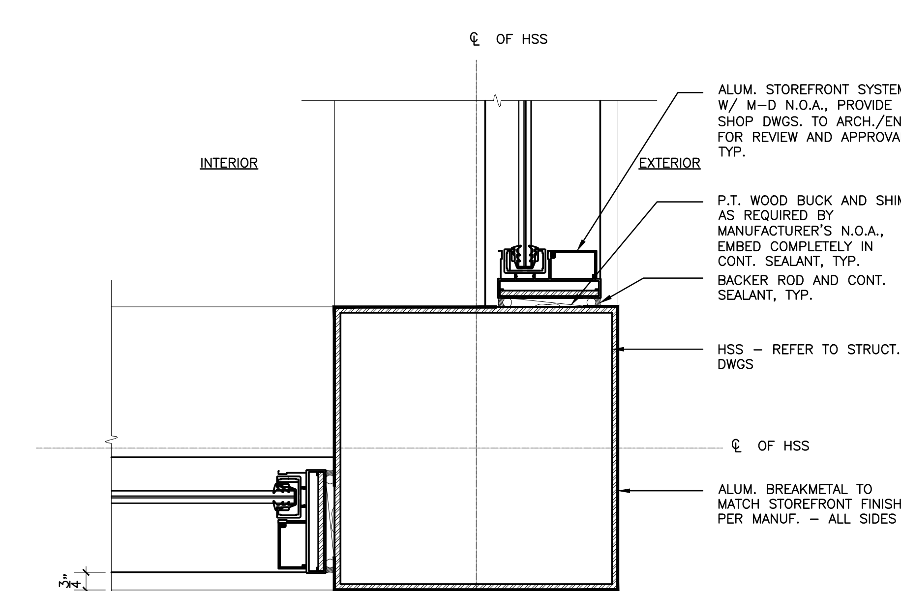
12 A-504 SLIDING GLASS DOOR - CORNER DETAIL SCALE: 3"=1'-0"
