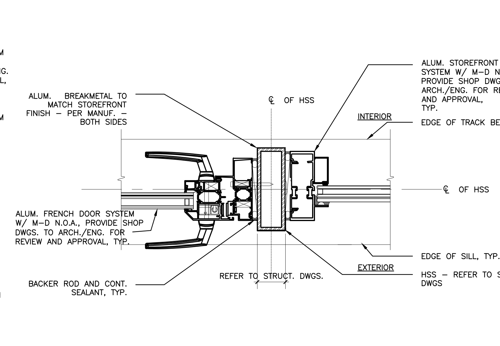
8 A-504 FRENCH DOOR - JAMB DETAIL @ TUBE STEEL SCALE: 3"=1'-0"
