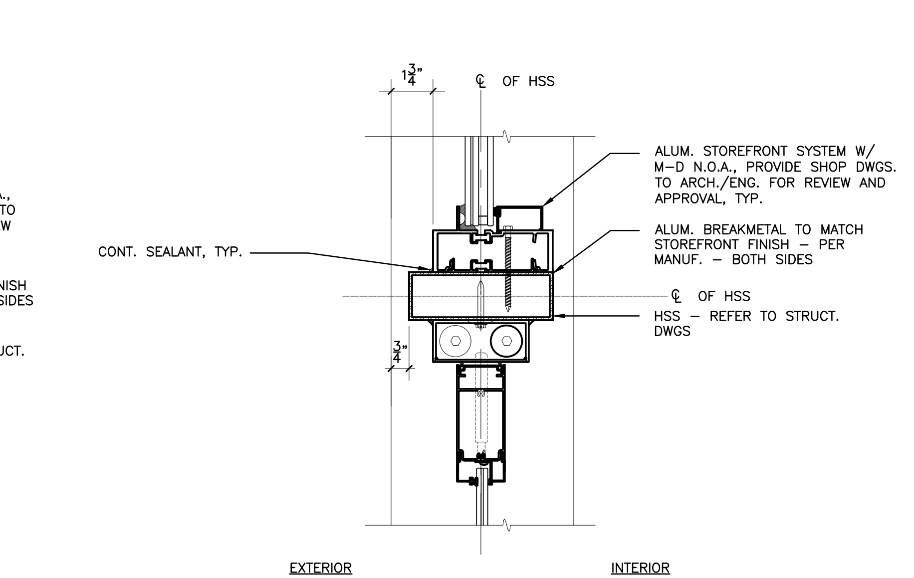
2 A-504 DOOR HEAD DETAIL - PIVOT DOOR CONNECTION SCALE: 3"=1'-0"
