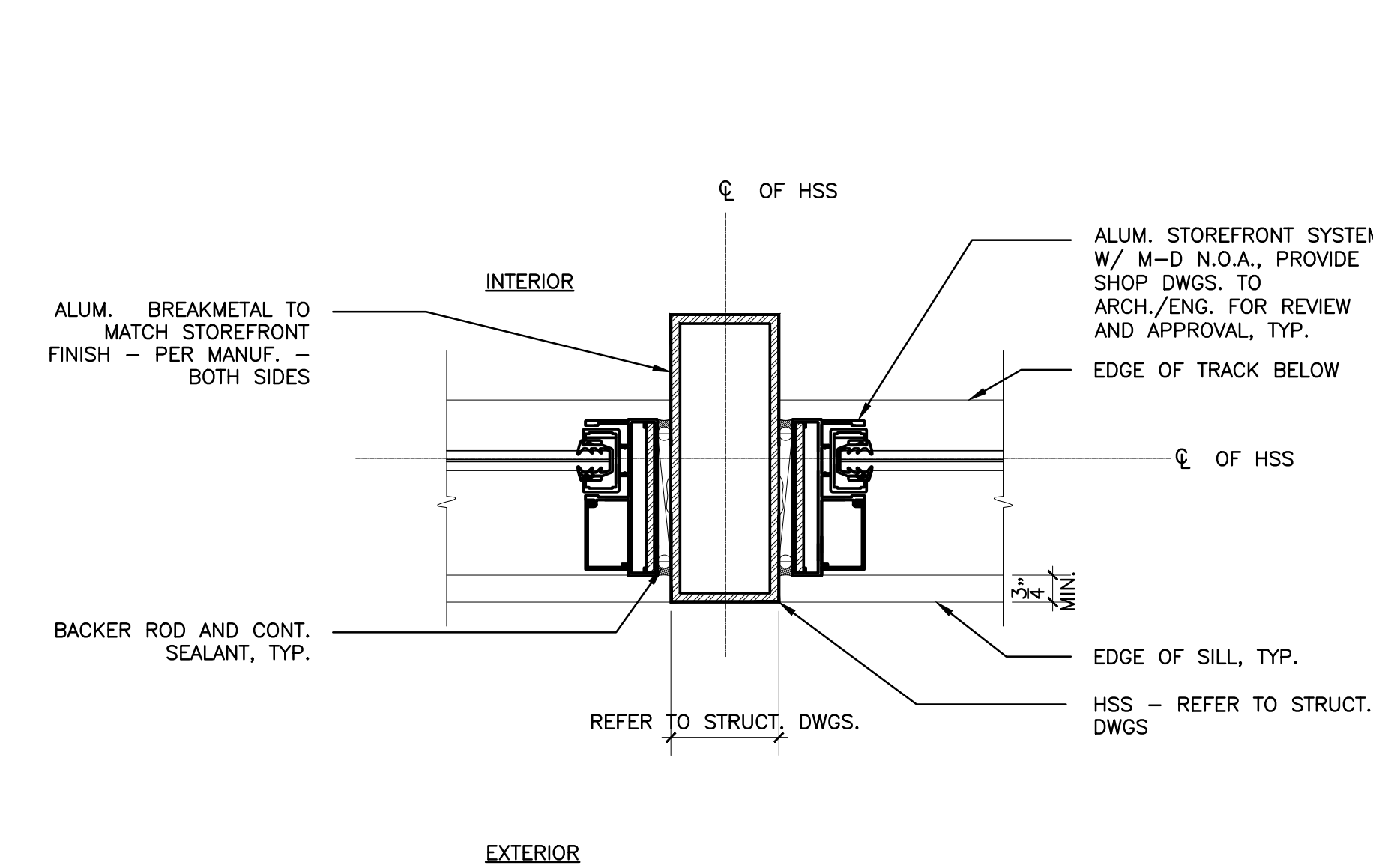
10 A-504 SLIDING GLASS DOOR - JAMB DETAIL SCALE: 3"=1'-0"
