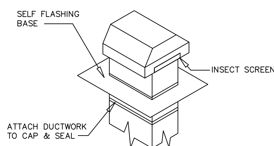
ROOF CAP TYPICAL DETAIL N.T.S.
