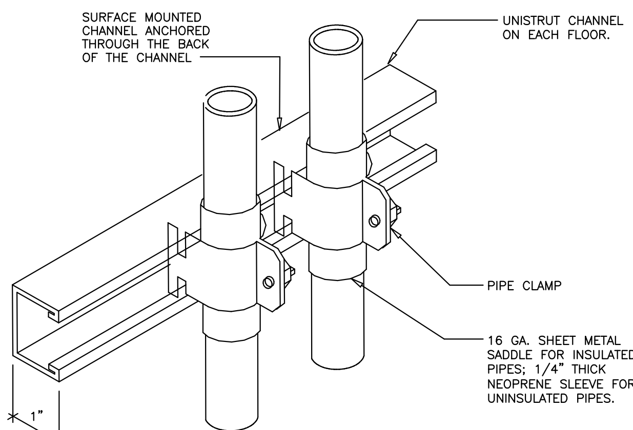
REFRIGERANT PIPE RISER WALL SUPPORT DETAIL N.T.S.
