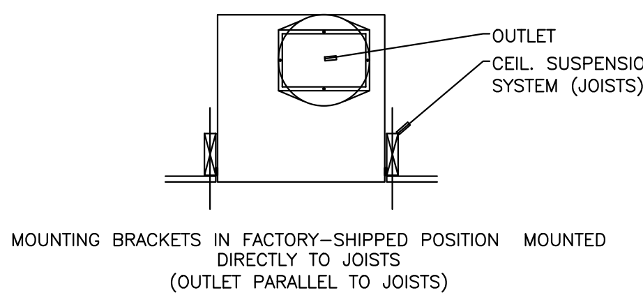
CEILING EXHAUST FAN TYPICAL INSTALLATION N.T.S.
