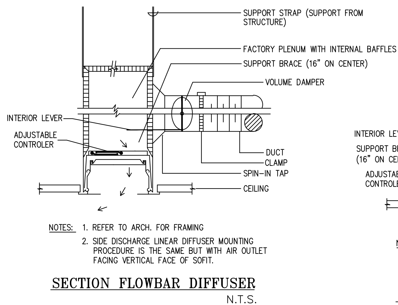
SECTION FLOWBAR DIFFUSER N.T.S.
