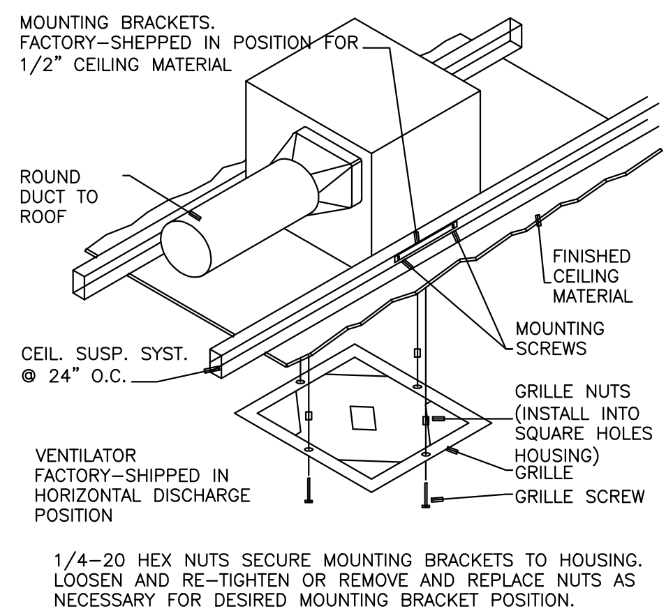
HVAC DUCT CONNECTION DETAILS N.T.S.
