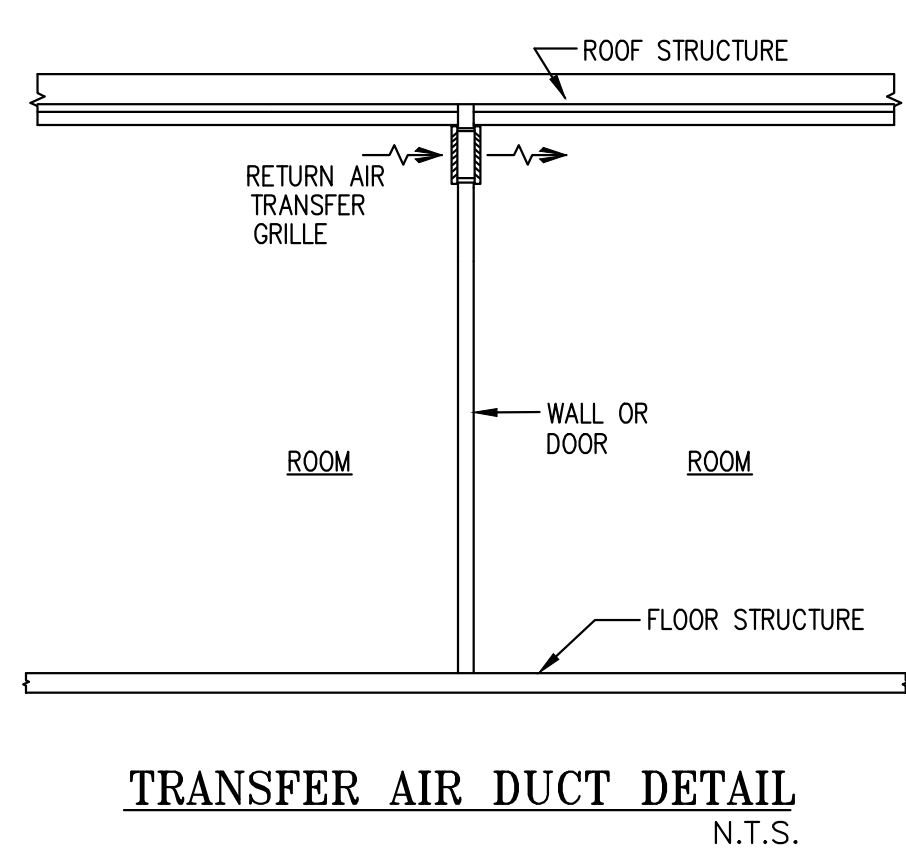
TRANSFER AIR DUCT DETAIL N.T.S.
