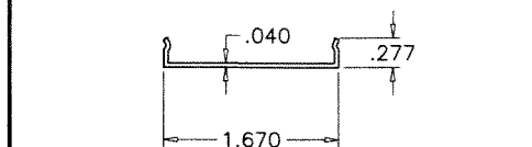
E2 FRAME SCREW COVER
