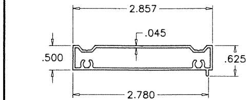
E5 FLUSH FRAME ADAPTER
