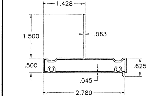
E6 FLUSH FRAME ADAPTER WITH FIN
