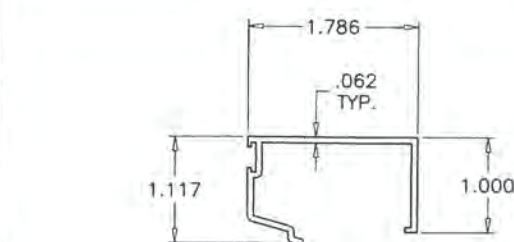
INTERMEDIATE HORIZONTAL
