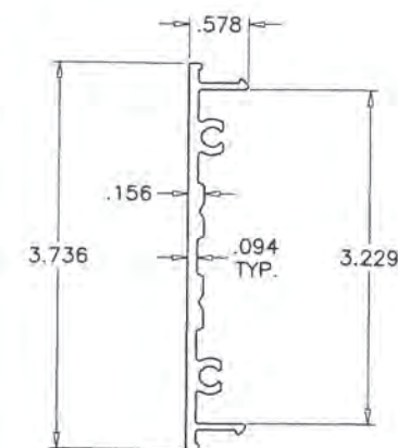
SHEAR CLIP
