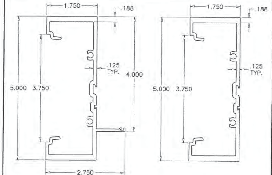
FRAME JAMB/MULLION
