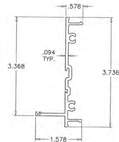
MULLION SNAP-IN MATE
