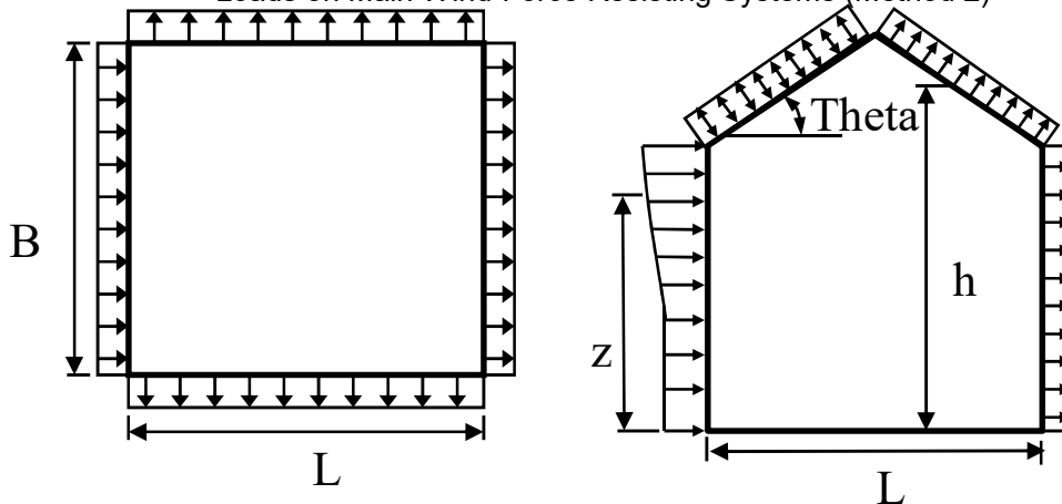
Figure 6-6 - External Pressure Coefficients, Cp
