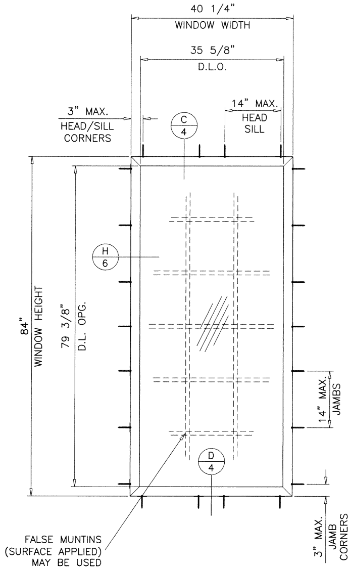
FIXED (O) TYPICAL ELEVATION
