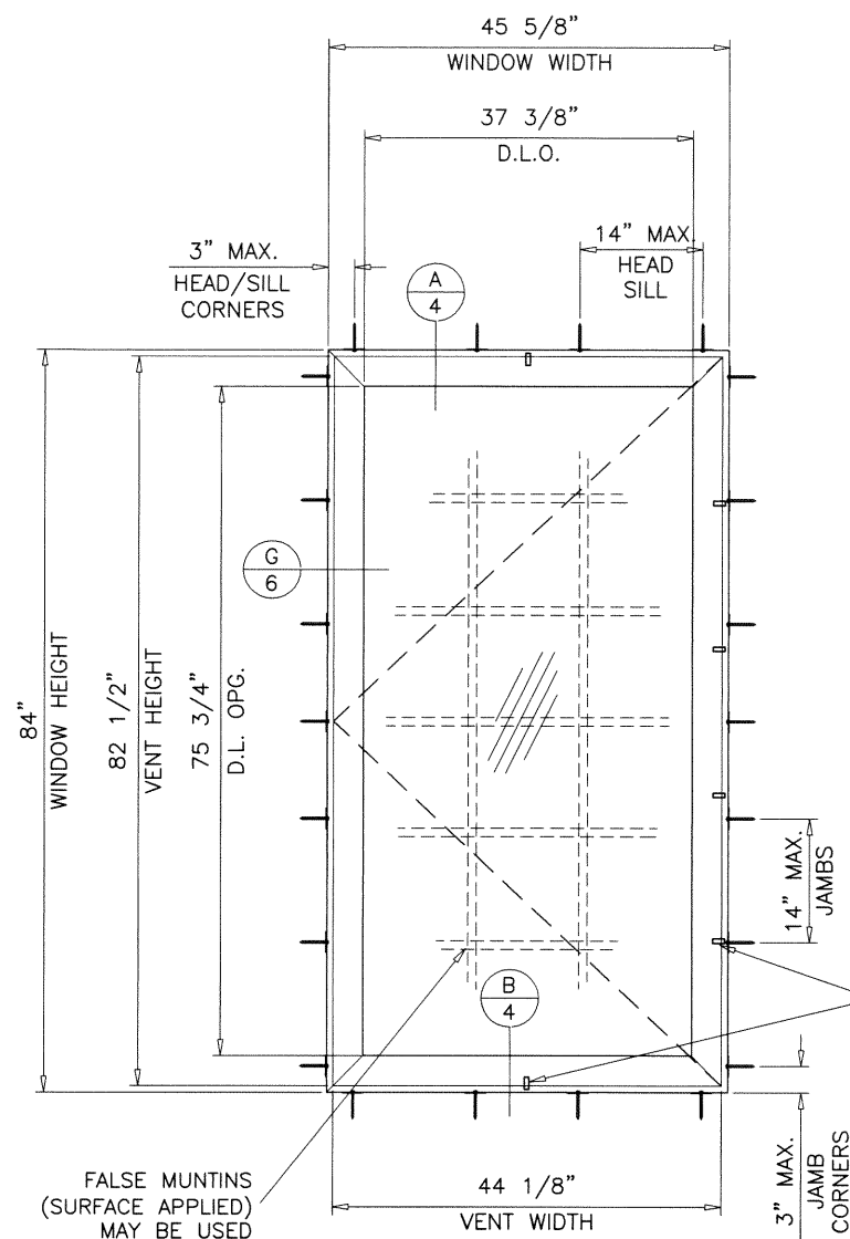
CASEMENT (X)
