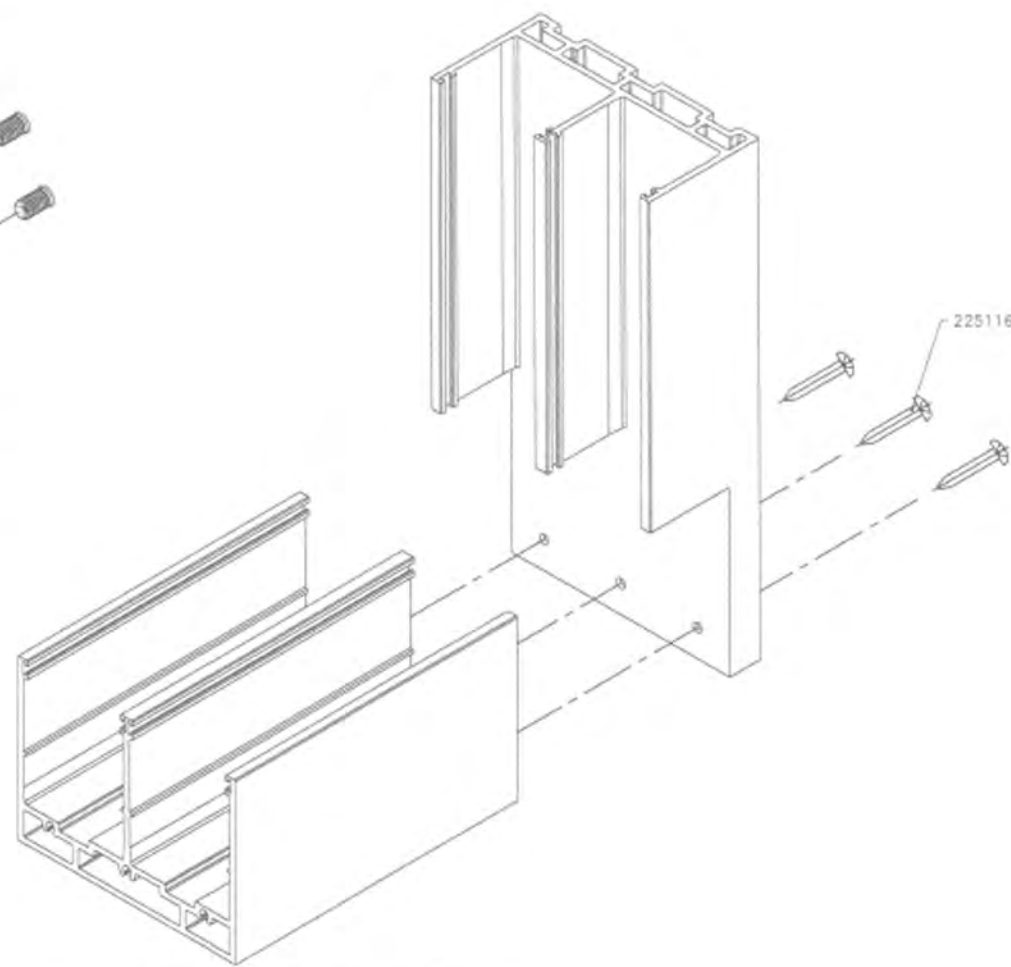
FRAME BOTTOM CORNER (2 TRACK FRAME)
