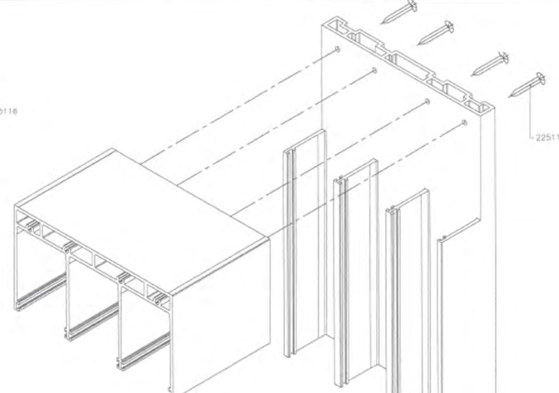
FRAME TOP CORNER (3 TRACK FRAME)
