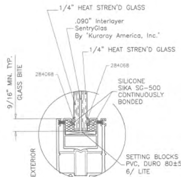
GLASS TYPE 'C' 9/16" OVERALL LAMINATED GLASS
