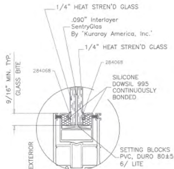
GLASS TYPE 'B' 9/16" OVERALL LAMINATED GLASS
