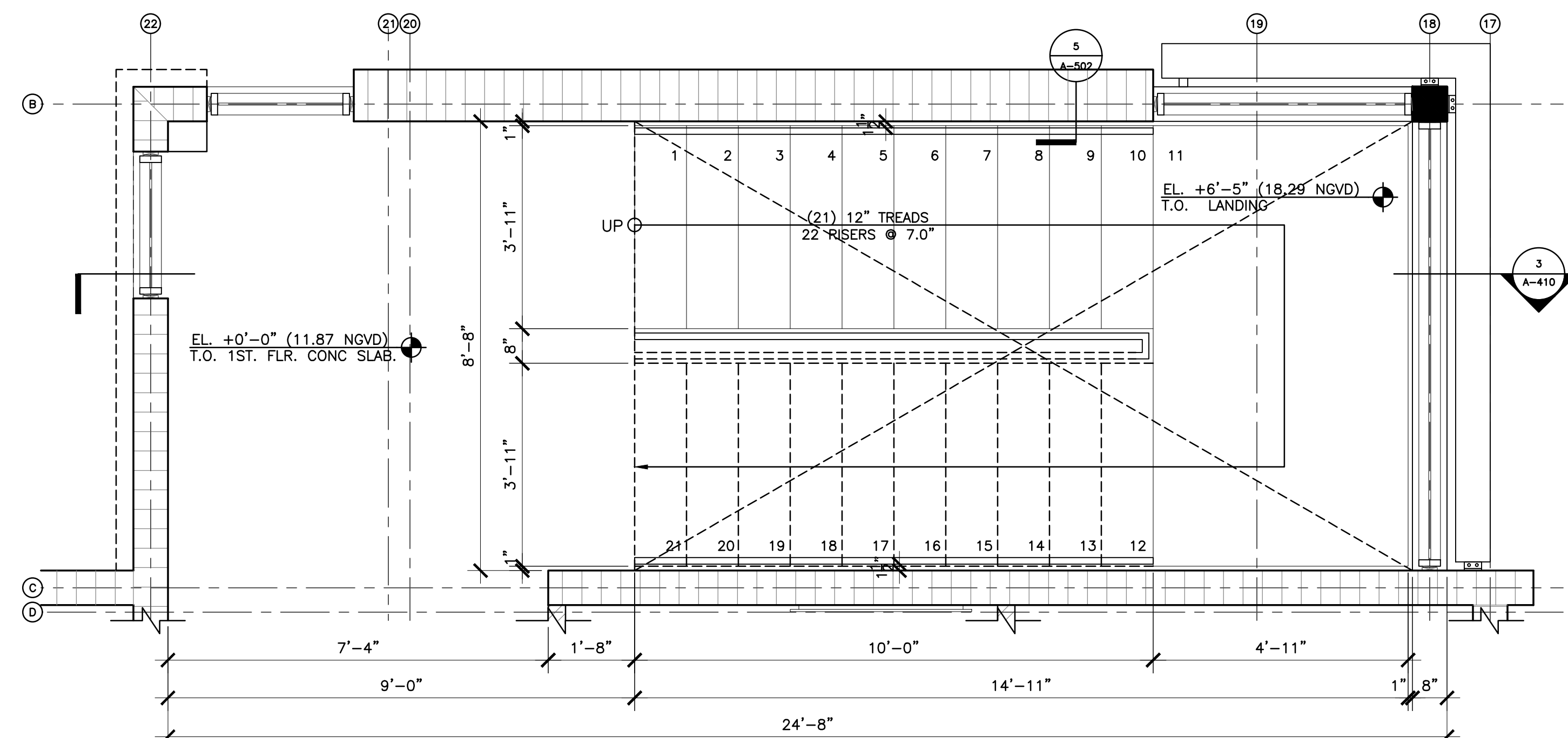
1 FIRST FLOOR STAIR PLAN A-410 SCALE: 1/2"=1'-0"
