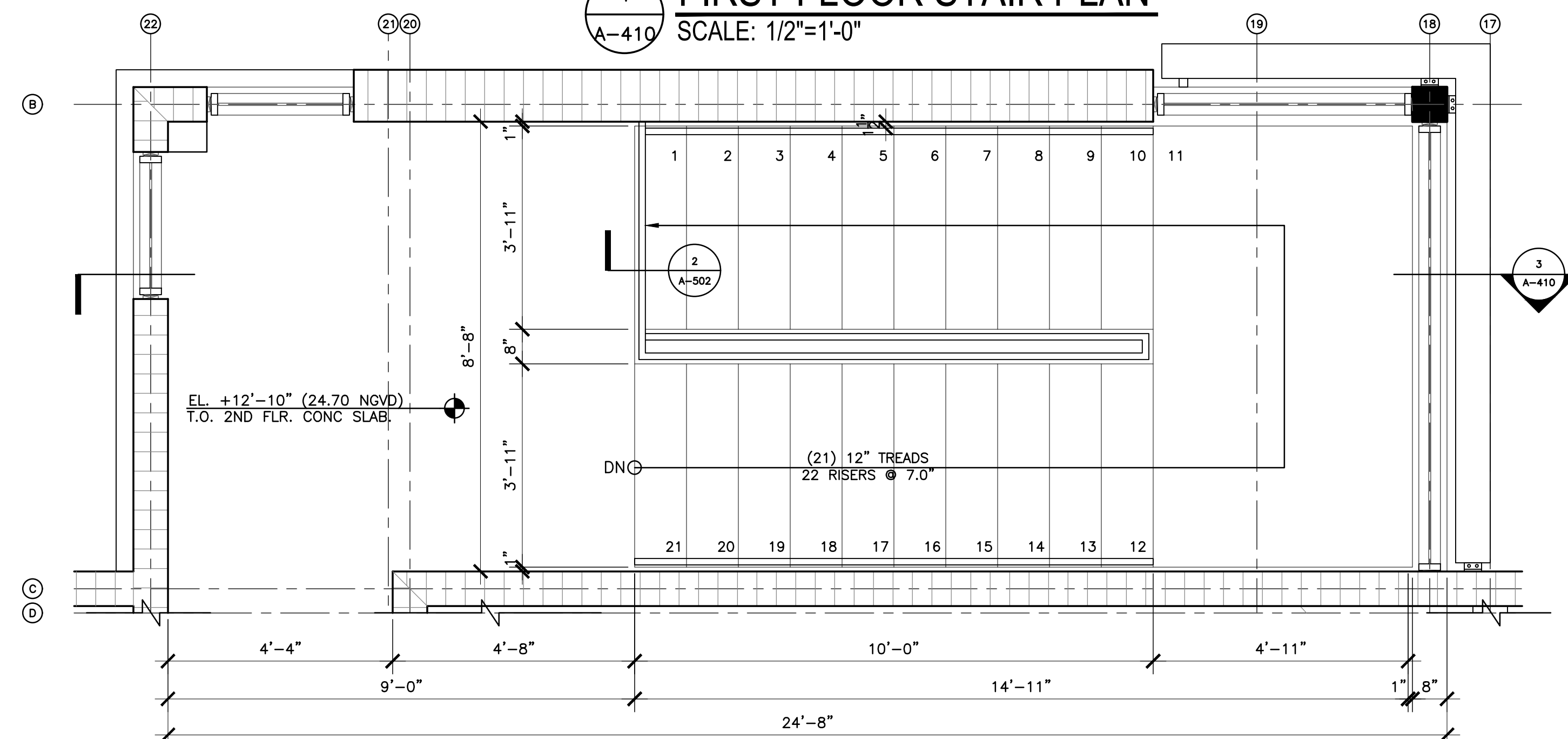
2 SECOND FLOOR STAIR PLAN A-410 SCALE: 1/2"=1'-0"
