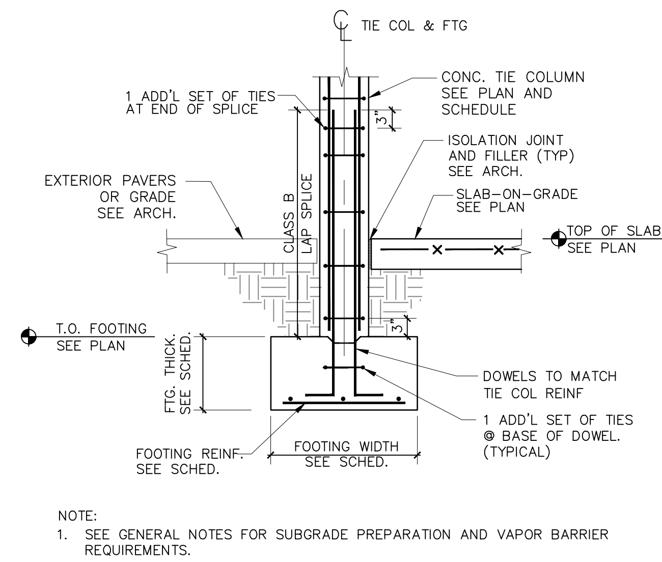
TYPICAL DETAIL CONCRETE TIE COLUMN TO WALL FOOTING CONNECTION
