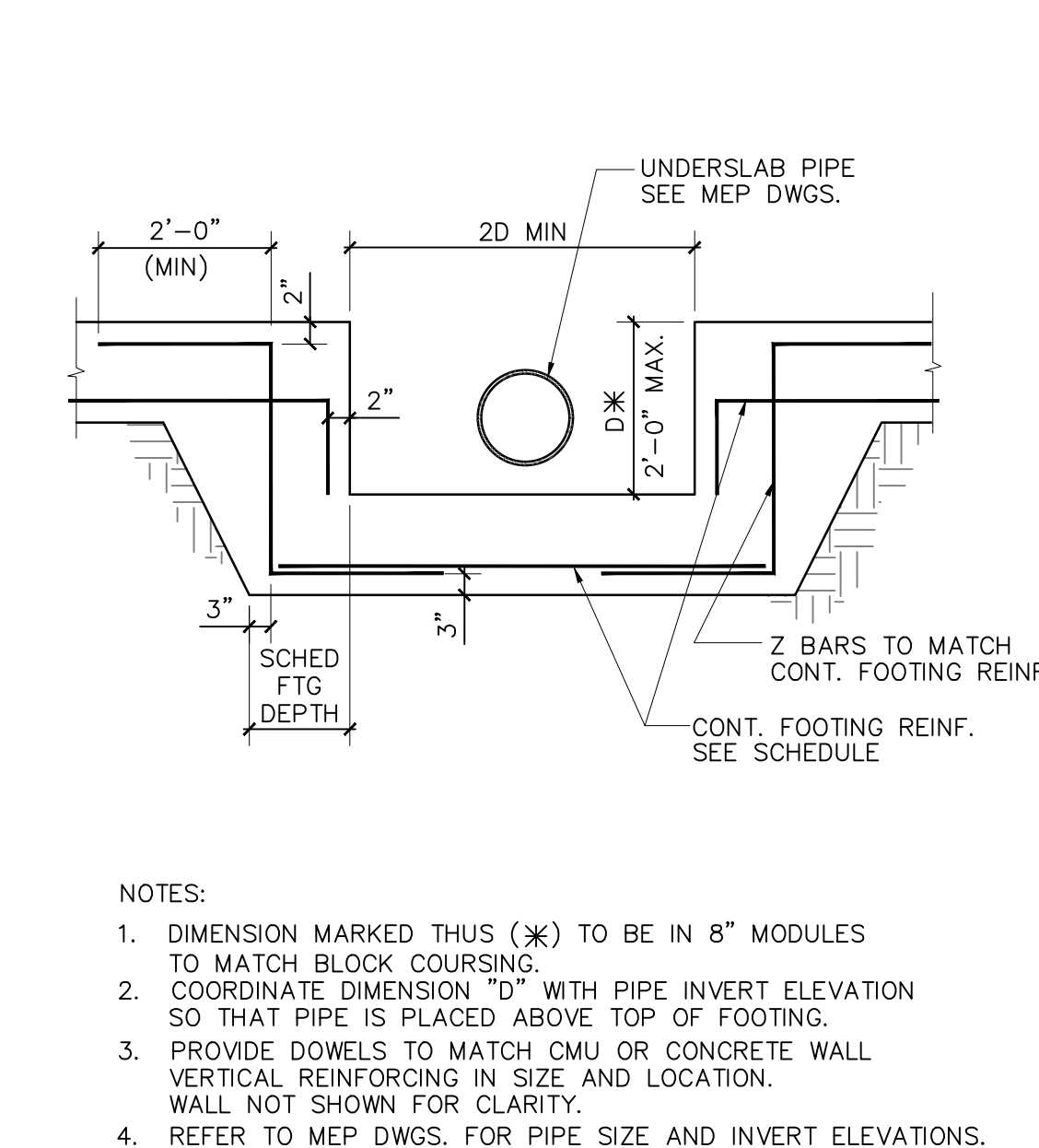
TYPICAL DETAIL STEP FOOTING AT UNDERSLAB PIPE PENETRATIONS
