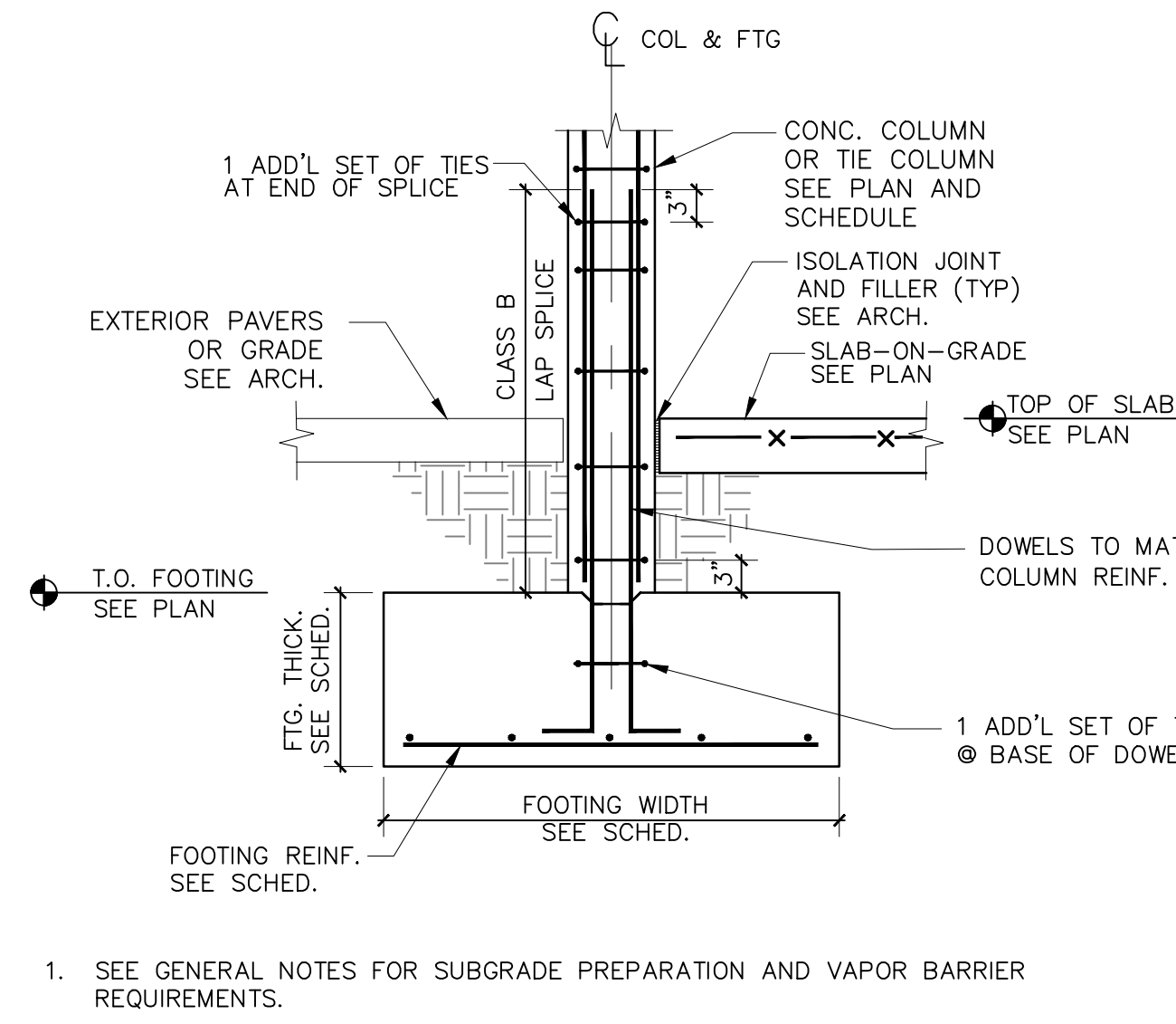
TYPICAL DETAIL CONCRETE COLUMN OR TIE COLUMN TO FOOTING CONNECTION
