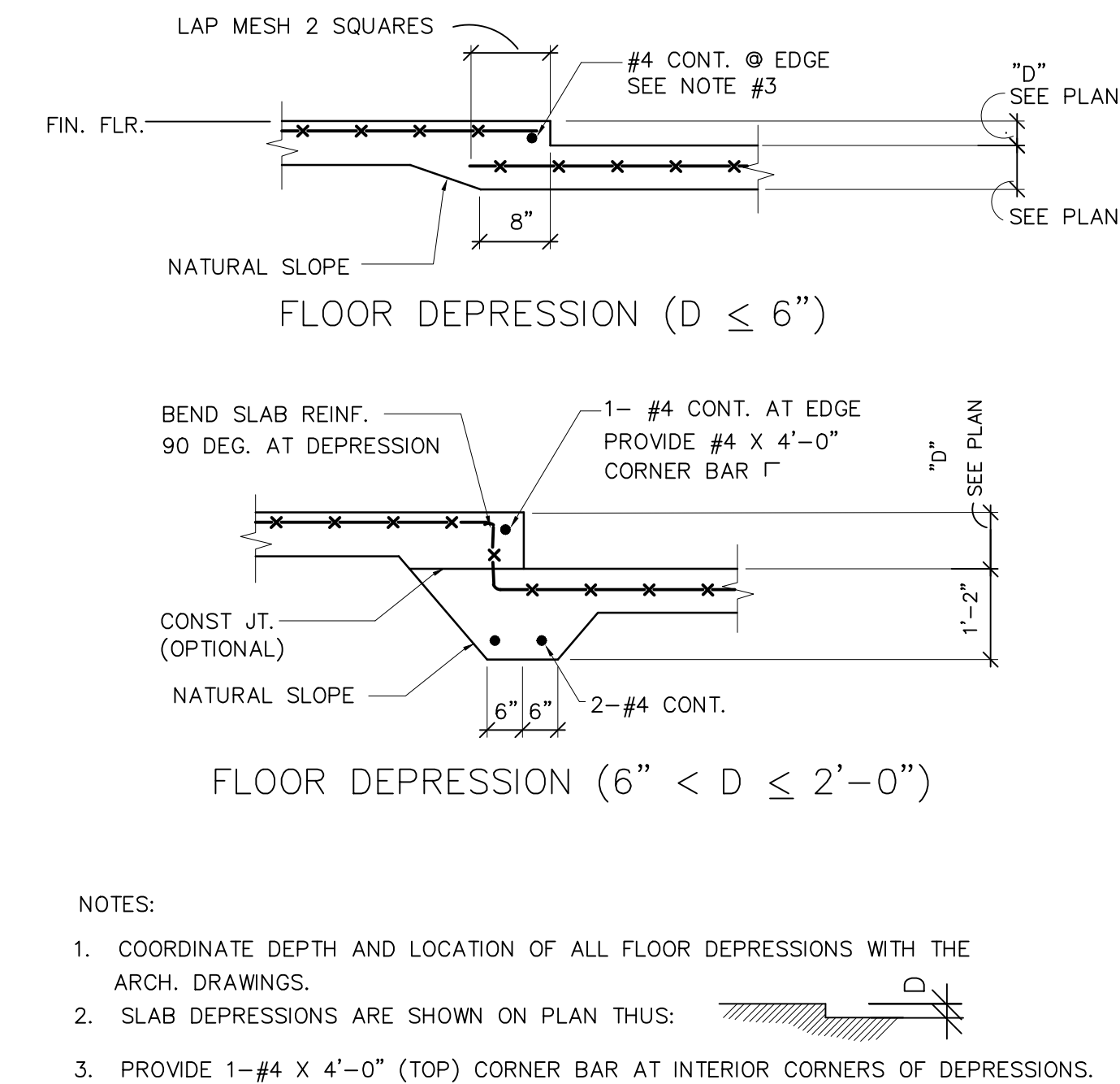
TYPICAL DETAIL FLOOR DEPRESSIONS SLAB-ON-GRADE
