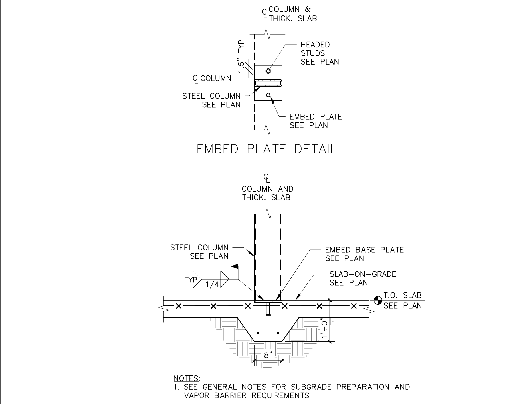
TYPICAL DETAIL STEEL COLUMN TO THICKENED SLAB CONNECTION
