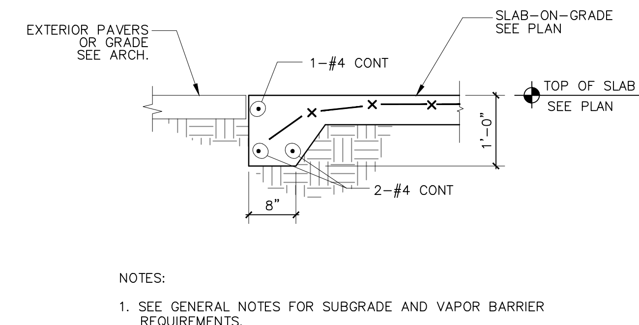
TYPICAL DETAIL THICKENED SLAB EDGE SLAB-ON-GRADE
