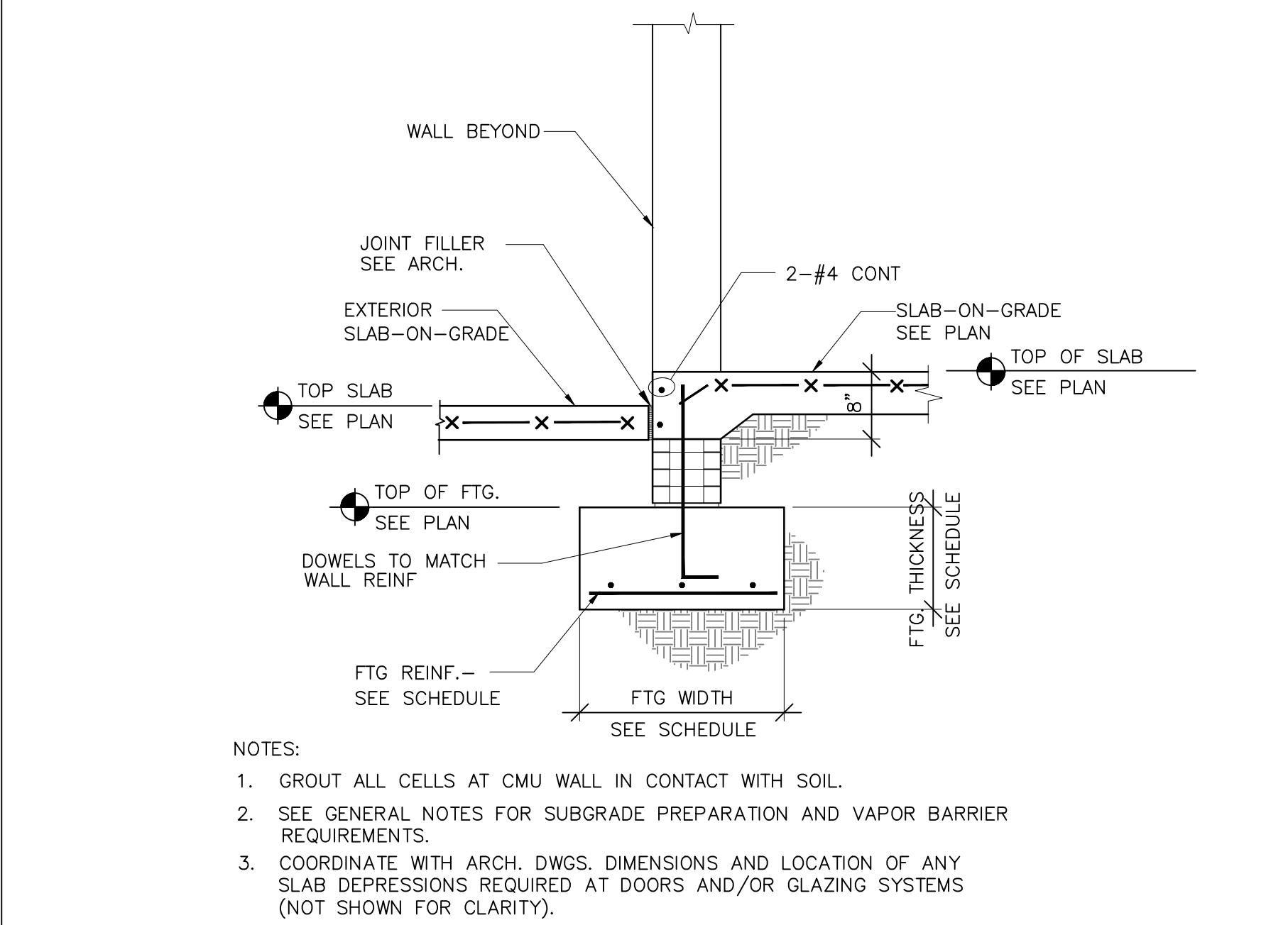
TYPICAL DETAIL CMU WALL TO FOOTING CONNECTION AT EXTERIOR DOOR OPENING
