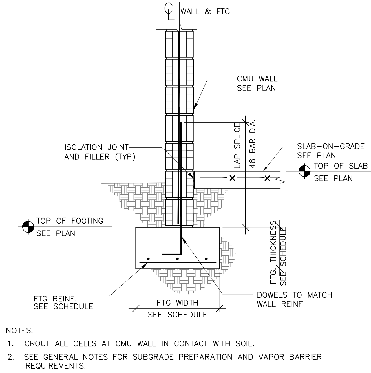
TYPICAL DETAIL EXTERIOR LOAD-BEARING CMU WALL TO FOOTING CONNECTION
