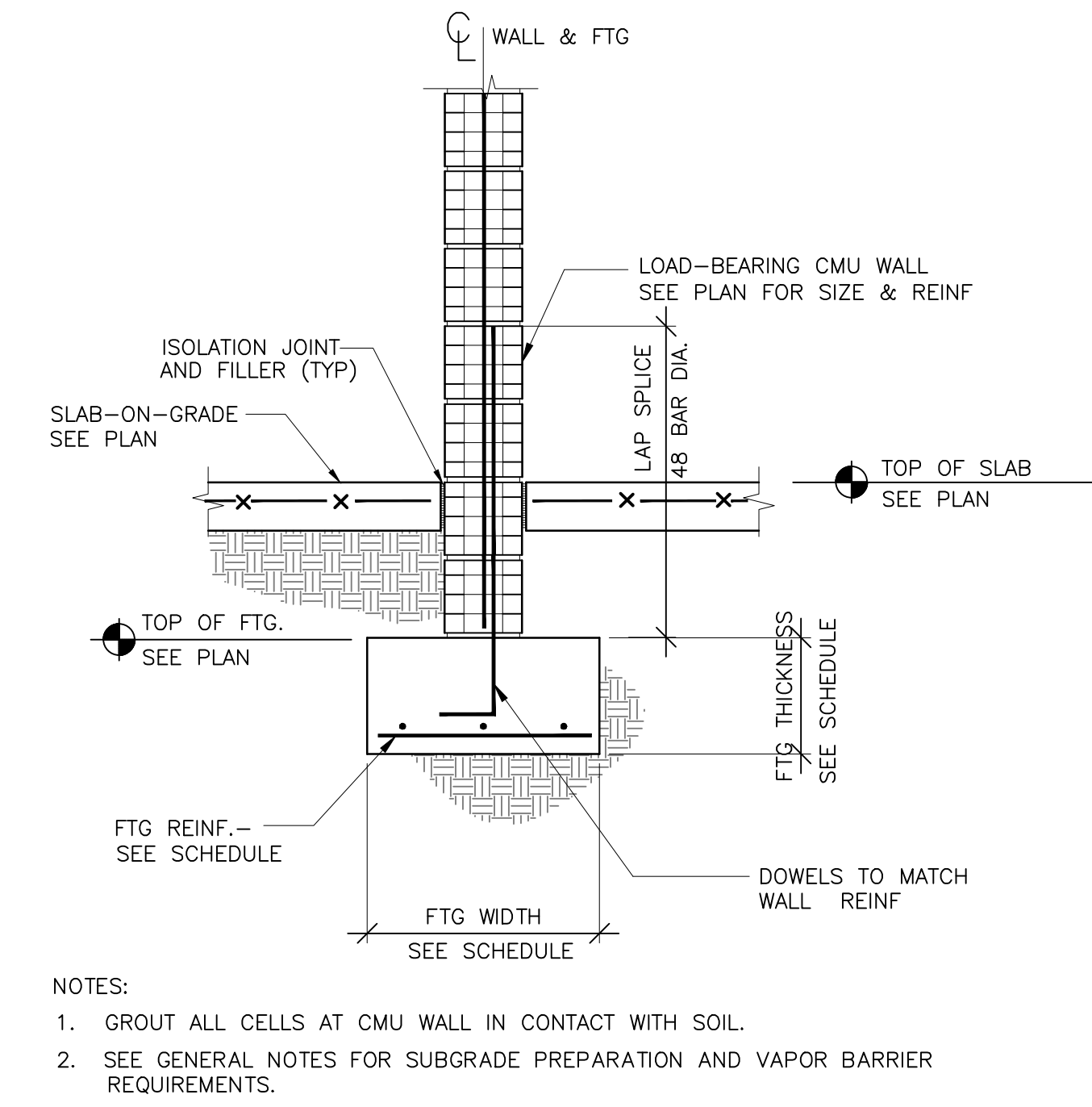
TYPICAL DETAIL INTERIOR LOAD-BEARING CMU WALL TO FOOTING CONNECTION
