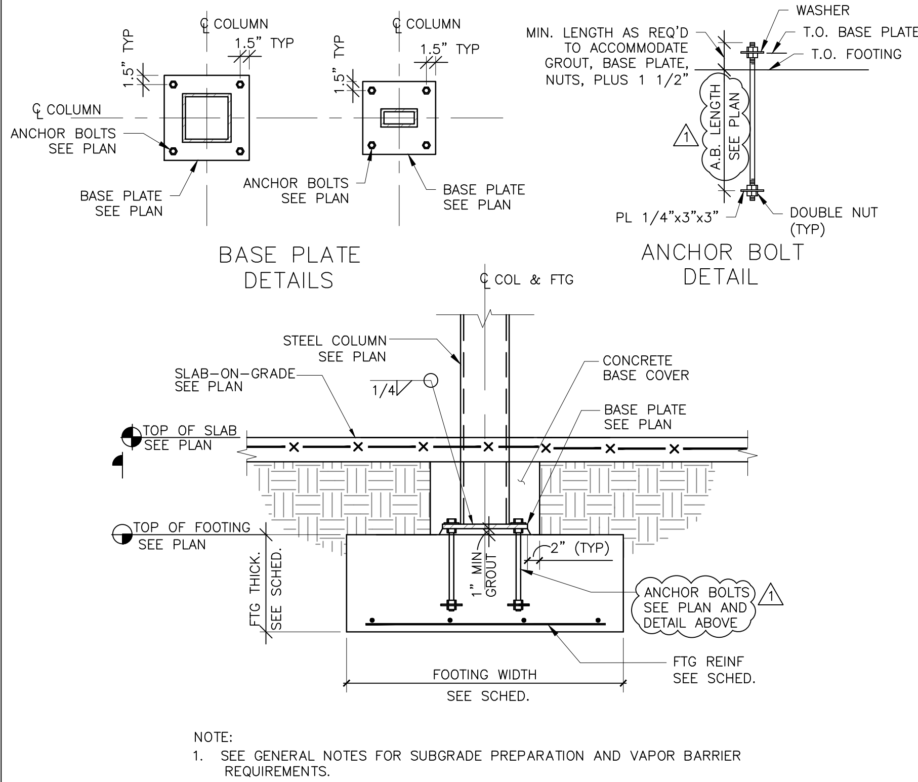
TYPICAL DETAIL STEEL COLUMN TO FOOTING CONNECTION
