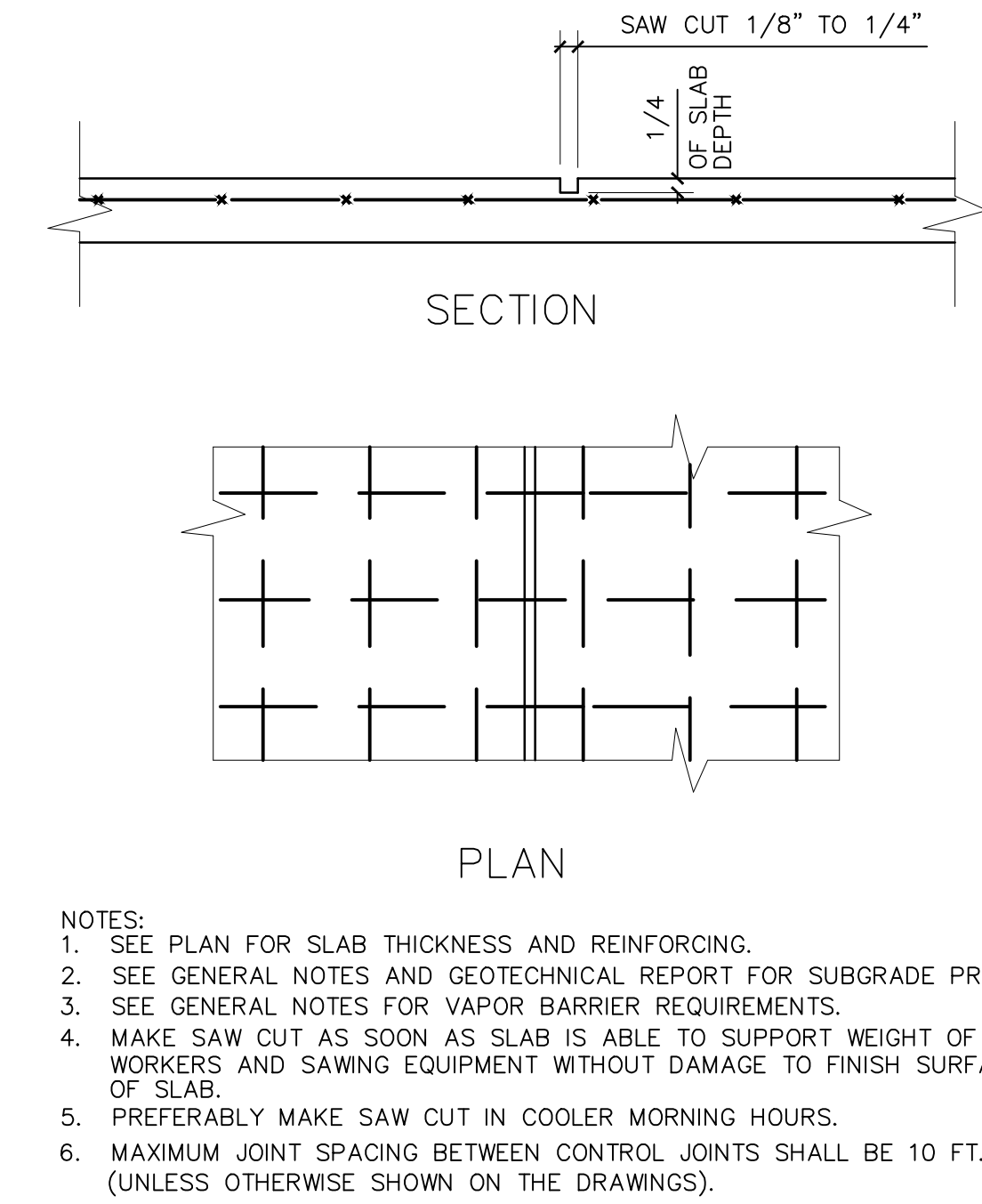
TYPICAL DETAIL CONTROL JOINT SLAB-ON-GRADE
