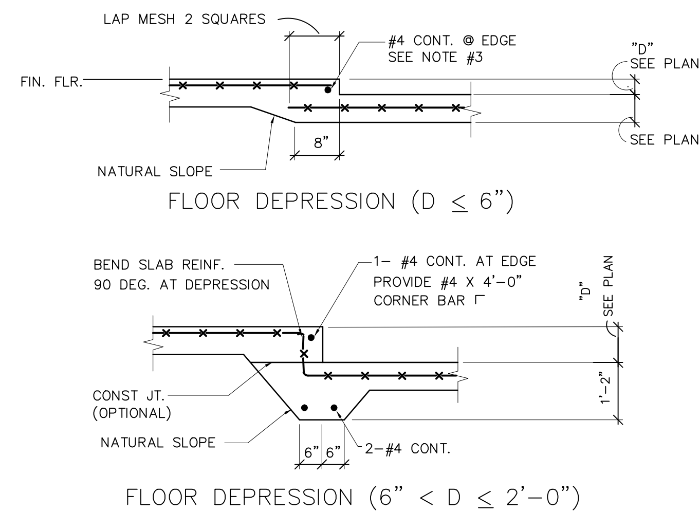
TYPICAL DETAIL FLOOR DEPRESSIONS SLAB-ON-GRADE
