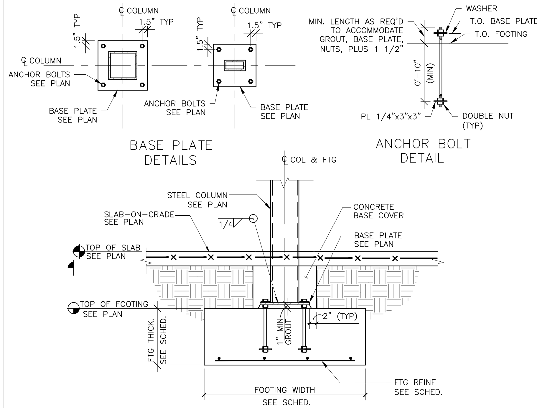
TYPICAL DETAIL STEEL COLUMN TO FOOTING CONNECTION
