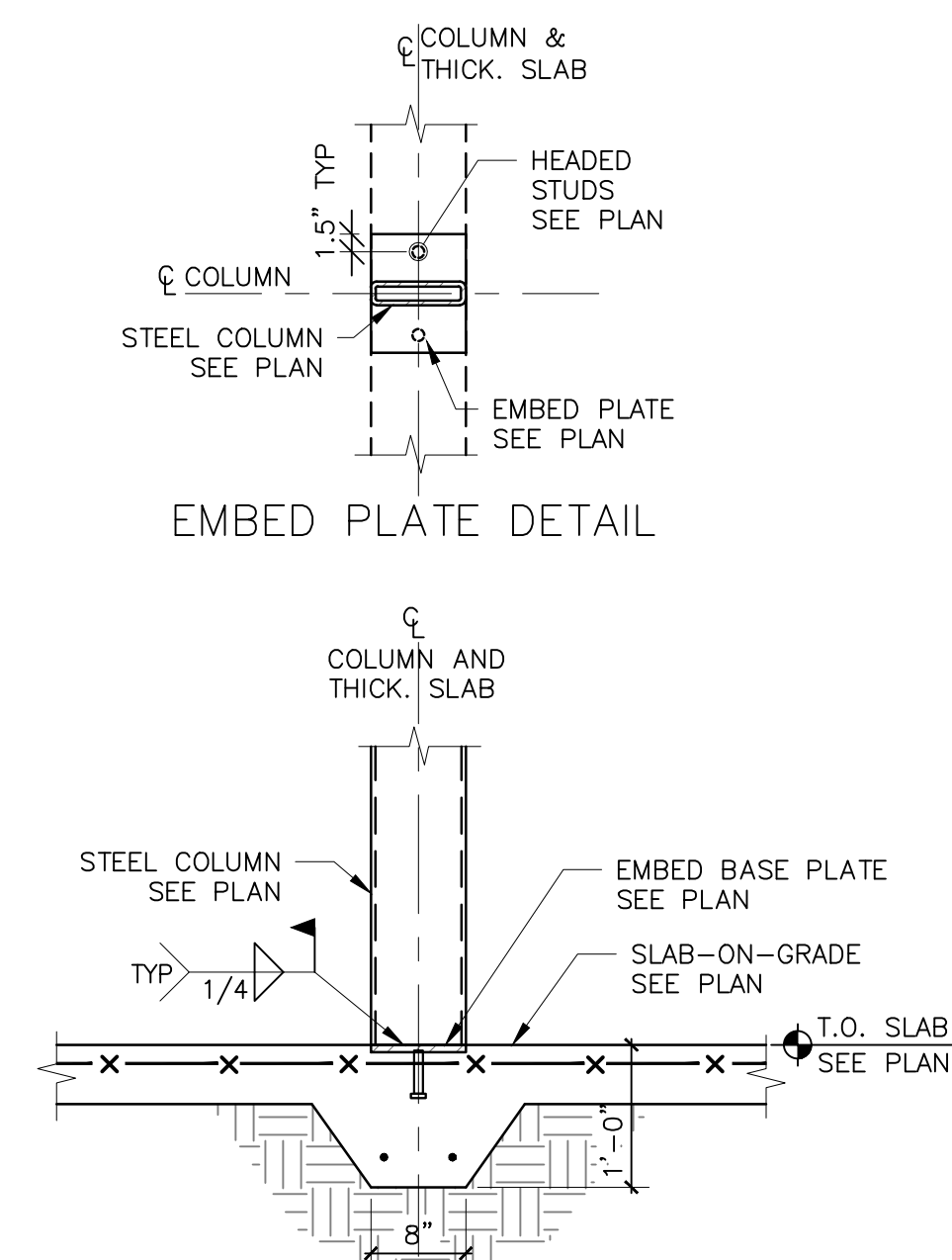
TYPICAL DETAIL STEEL COLUMN TO FOOTING CONNECTION
