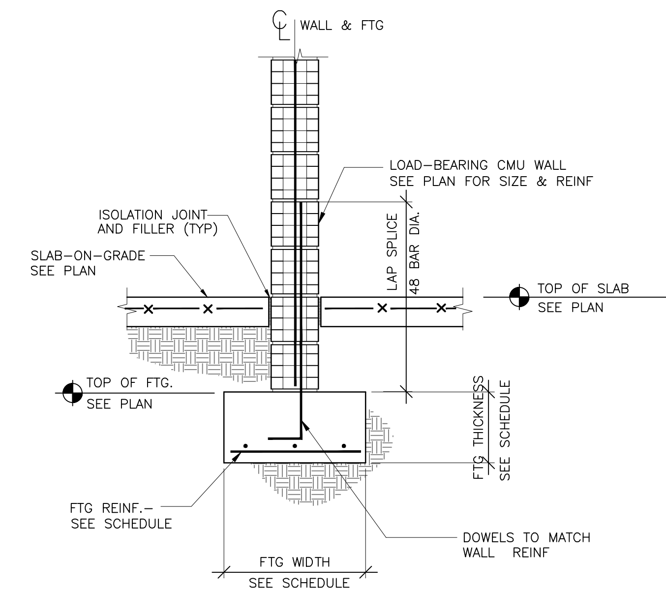
TYPICAL DETAIL INTERIOR LOAD-BEARING CMU WALL TO FOOTING CONNECTION
