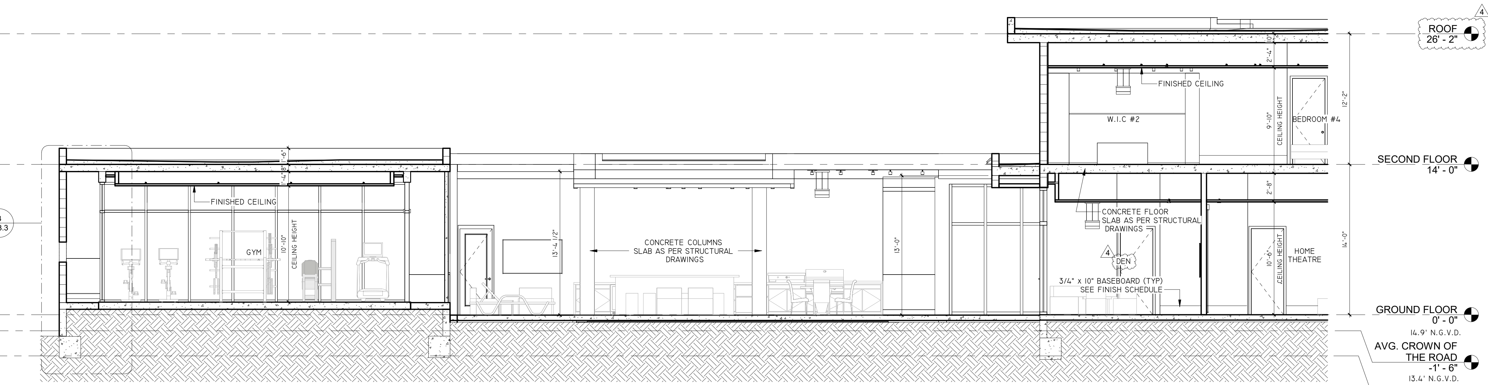
3 SECTION E-E - CALLOUT 2 3/16" = 1'-0"
