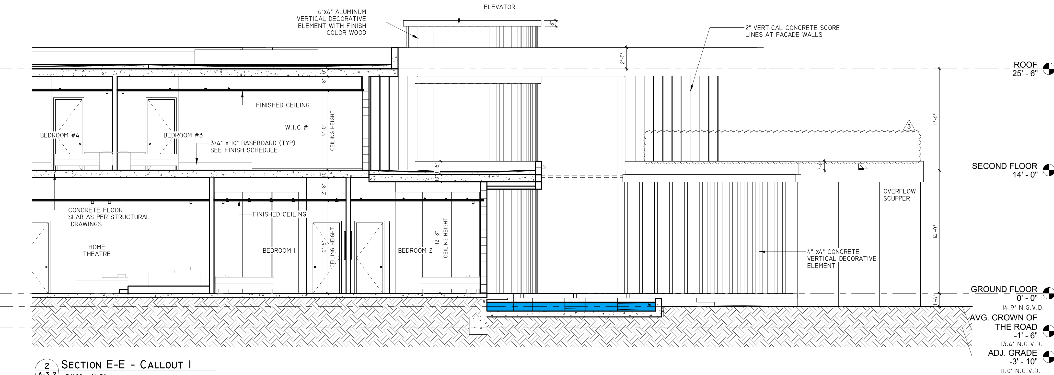
1 SECTION E-E 1/8" = 1'-0"
