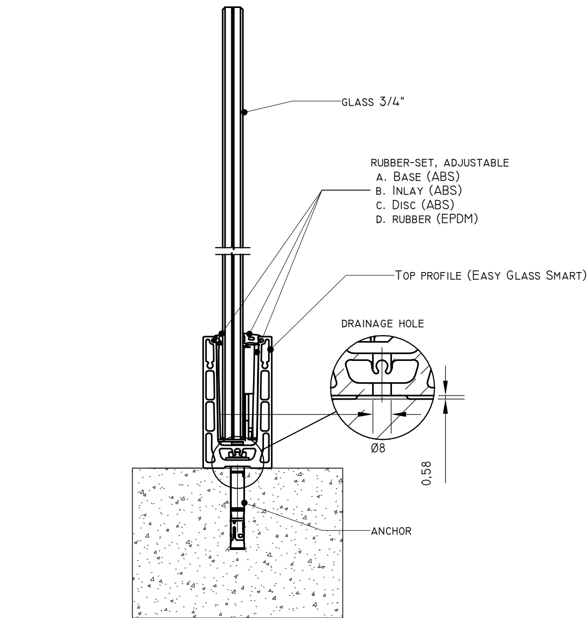
2 GLASS RAILING & ANCHOR DETAIL A-6.3 3/8" = 1'-0"
