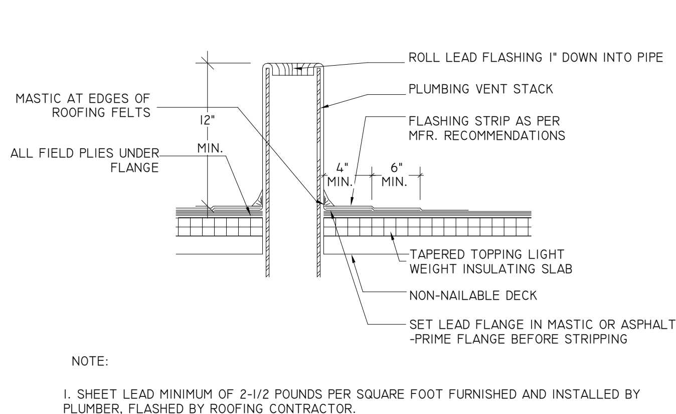
8 VENT THRU ROOF DETAIL A-6.3 1 1/2" = 1'-0"
