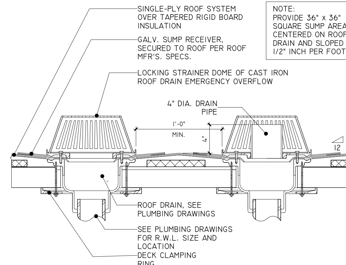
9 ROOF DRAIN/OVERFLOW A-6.3 1 1/2" = 1'-0"
