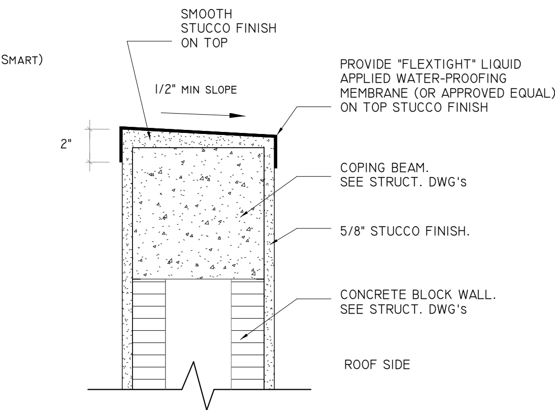
3 PARAPET COPING DETAIL A-6.3 3/8" = 1'-0"
