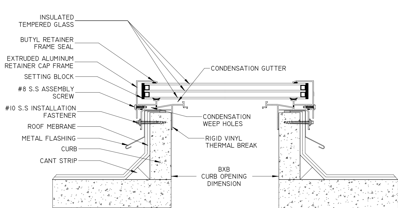
6 SKYLIGHTS A-6.3 1 1/2" = 1'-0"
