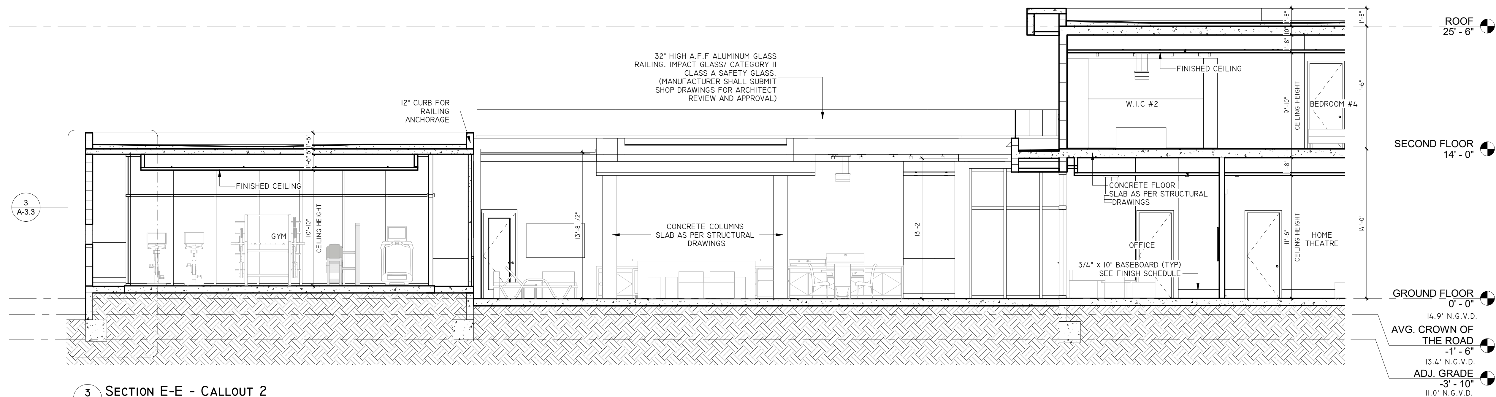
3 A-3.2 SECTION E-E - CALLOUT 2 3/16" = 1'-0"
