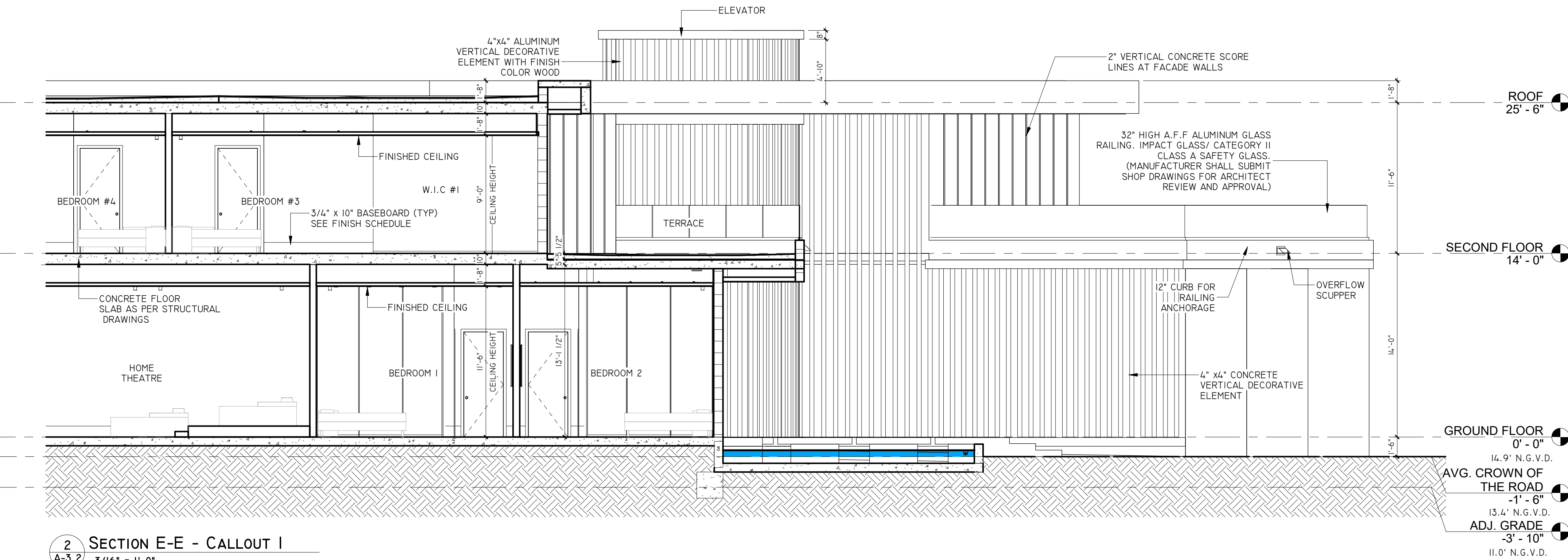
1 A-3.2 SECTION E-E 1/8" = 1'-0"
