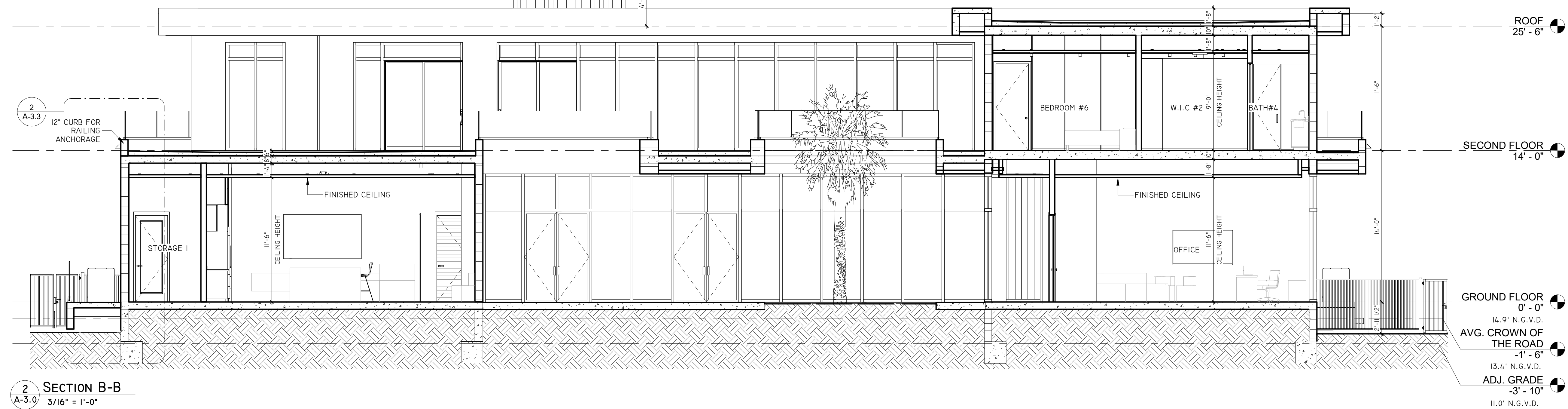
1 SECTION A-A A-3.0 3/16" = 1'-0"
