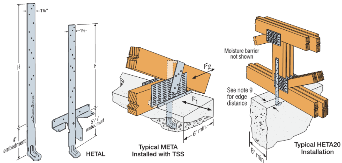
FIGURE 3: META / HETA / HHETA / HETAL Dimensions and Installation Details
