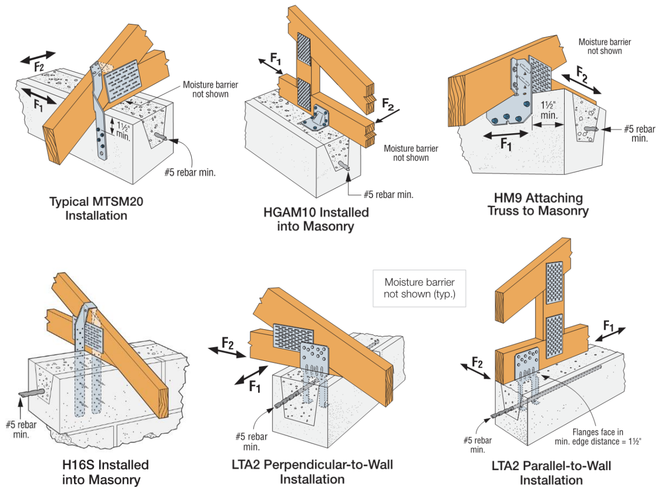
FIGURE 2: MTSM / HTSM / HM9 / HGAM10 / H16 / LTA2 Installation Details
