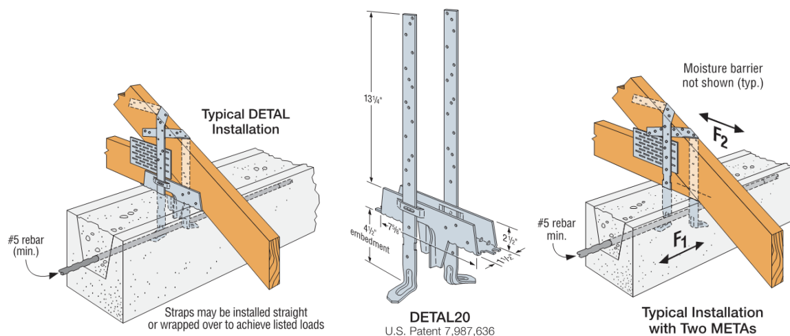
FIGURE 4: DETAL20 Dimensions and Double META / HETA / HHETA Installation Details
