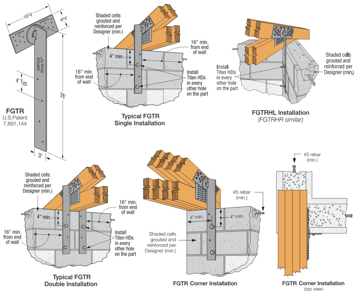
FIGURE 6: FGTR / FGTRHL / FGTRHR Dimensions and Installation Details
