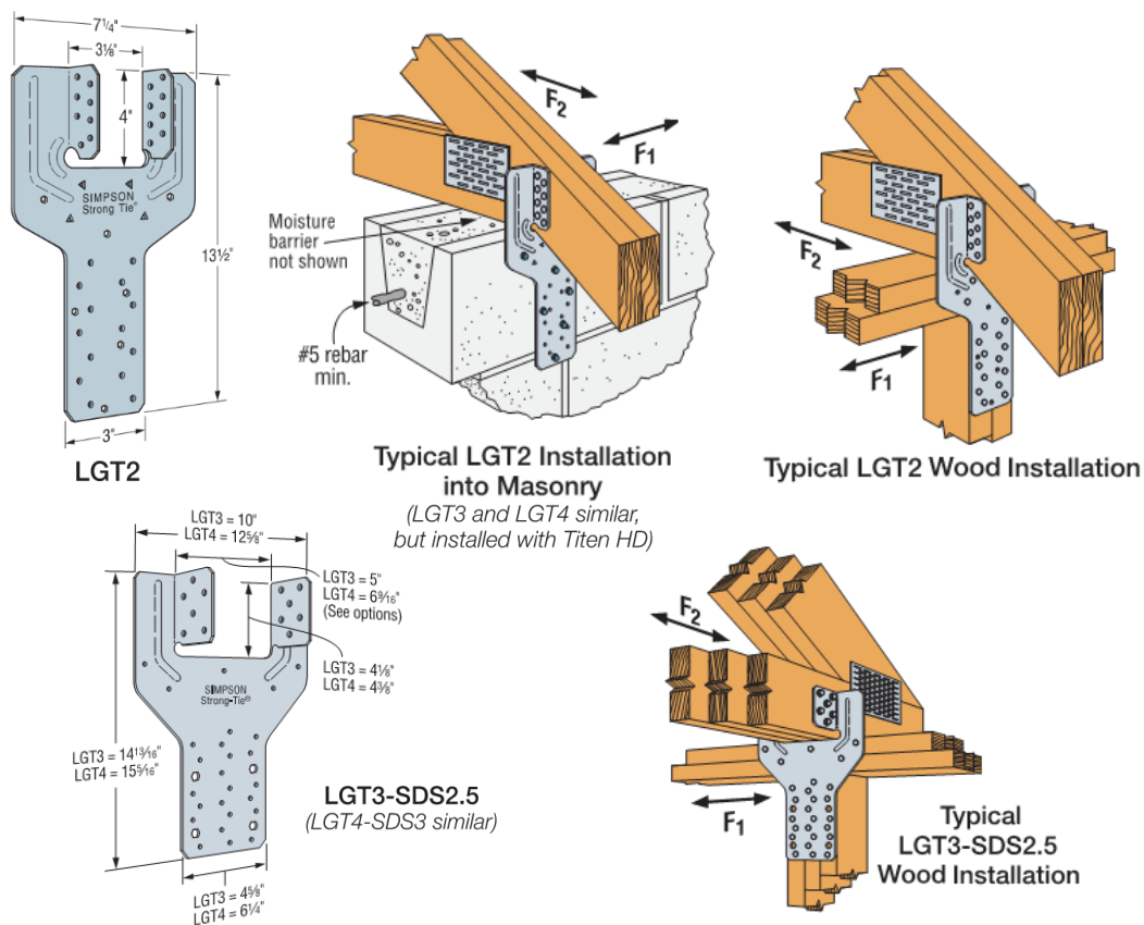
FIGURE 7: LGT2 / LGT3 / LGT4 Dimensions and Installation Details
