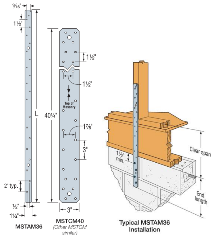
FIGURE 5: MSTAM / MSTCM Dimensions and Installation Details
