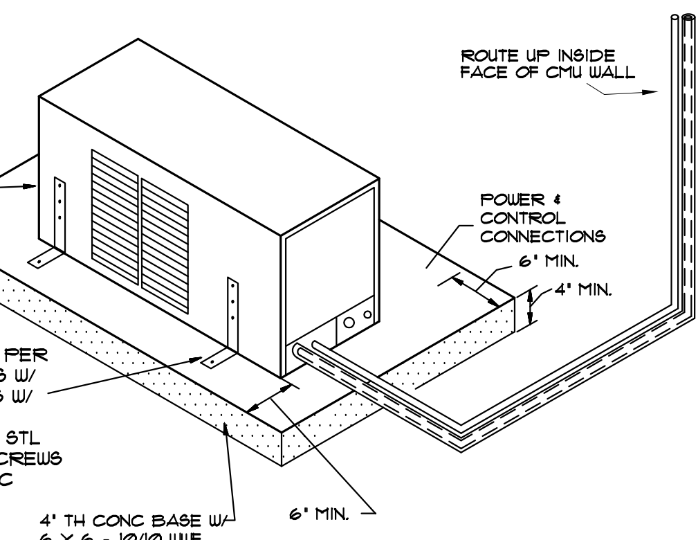
WINE COOLING UNIT N.T.S.
