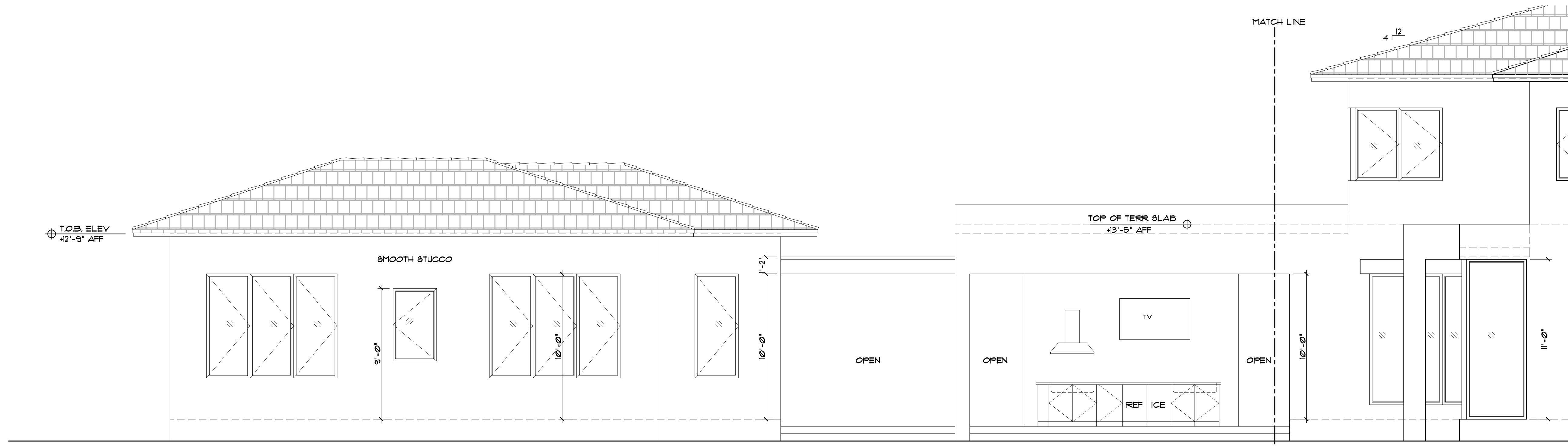
EAST SIDE ELEVATION SCALE: 1/4" = 1'-0"
