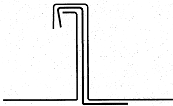
Before Seaming
