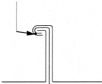
90 degree Seam w/Bostik Sealant
