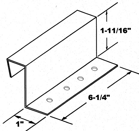
SERIES 1300 6" CLIP
