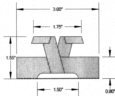
SERIES 1300 TWO-PIECE FLOATING CLIP
