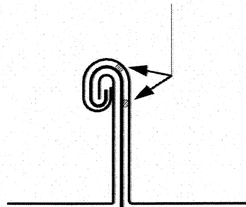
180 degree Seam w/ (2) beads of Bostik Sealant
