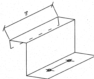
SERIES 1300 3" CLIP
