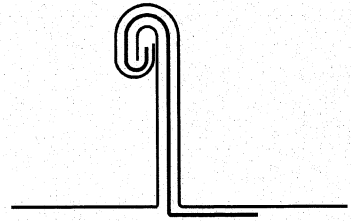
180 degree Seam
