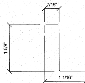
SERIES 1300 TWO-PIECE FLOATING CLIP
