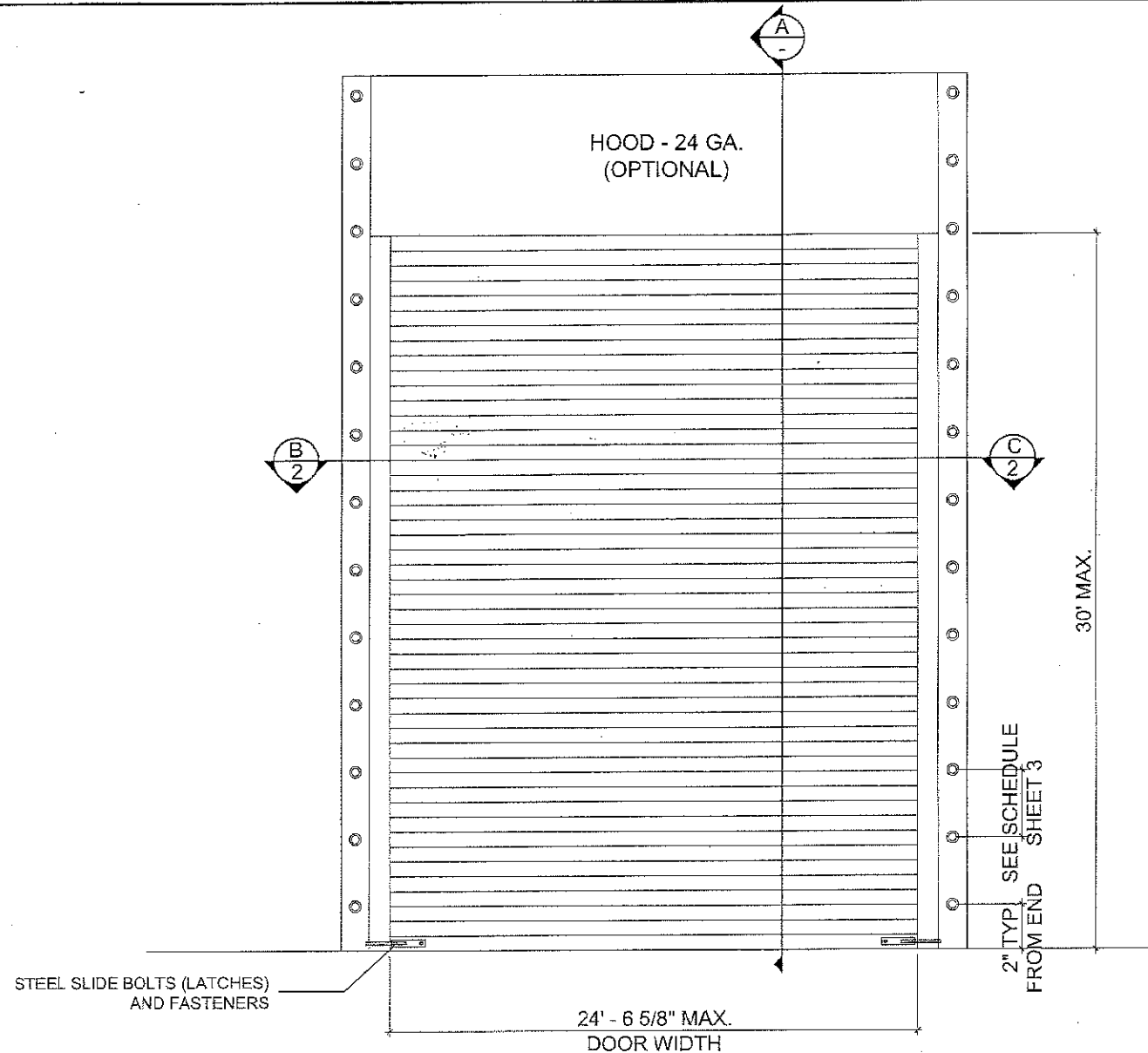
TYPICAL ELEVATION
