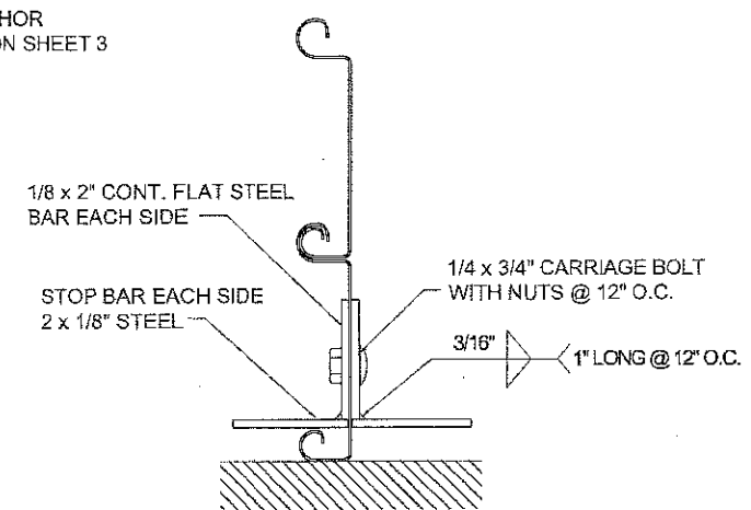
D BOTTOM BAR DETAIL
