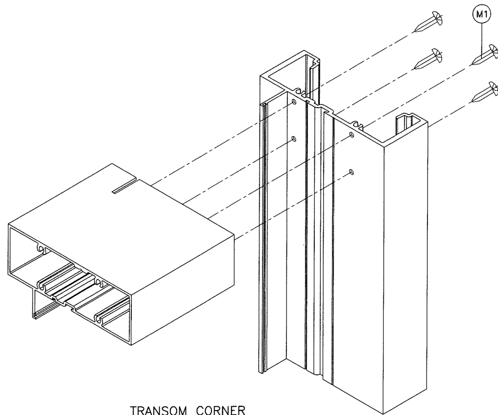
TRANSOM CORNER SERIES-8000 WINDOW WALL
