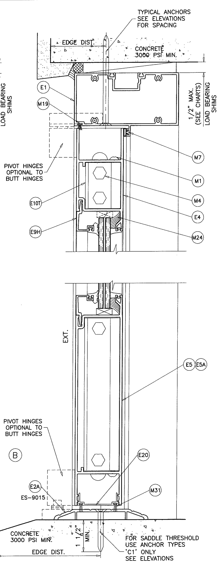
SADDLE THRESHOLD
