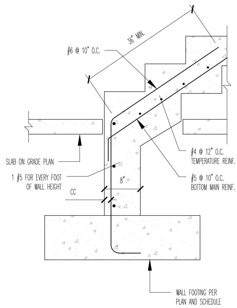
3 STAIR DETAIL FOUNDATION SCALE 3/4" = 1'-0"
