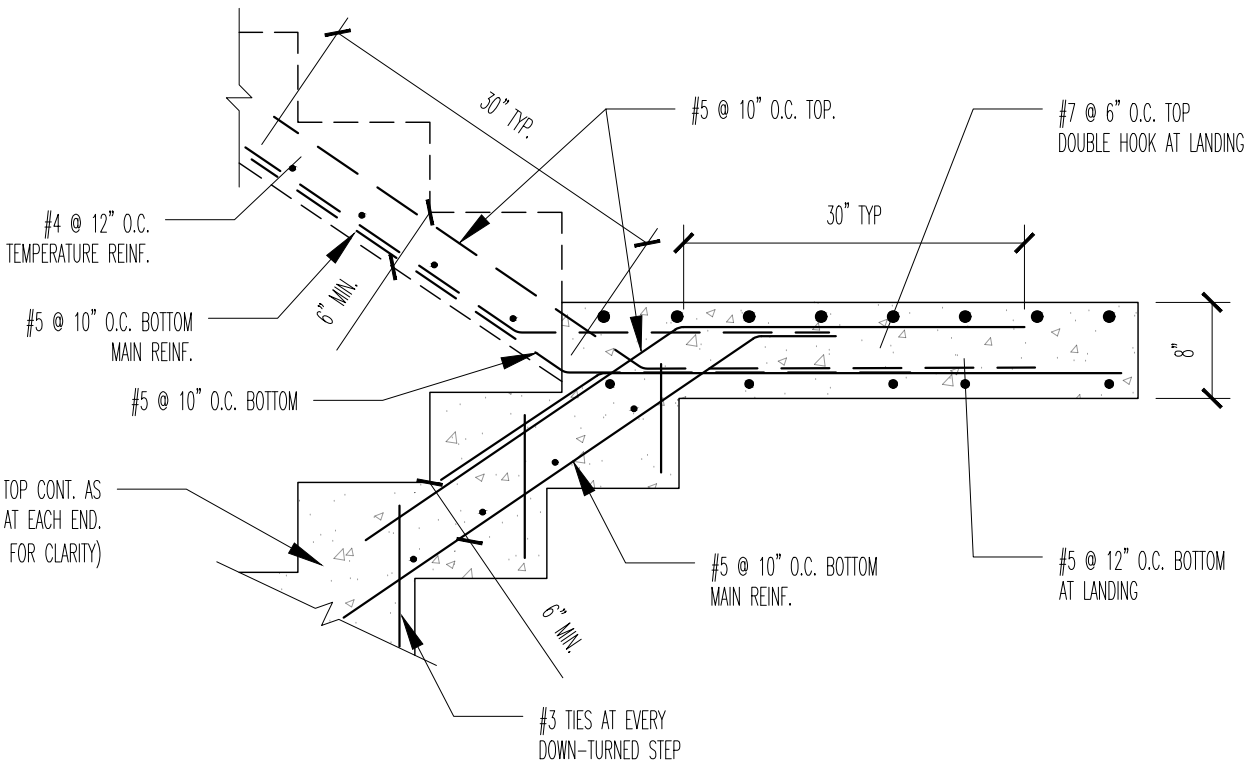
1 STAIR DETAIL INTERMEDIATE LANDING SCALE 3/4" = 1'-0"
