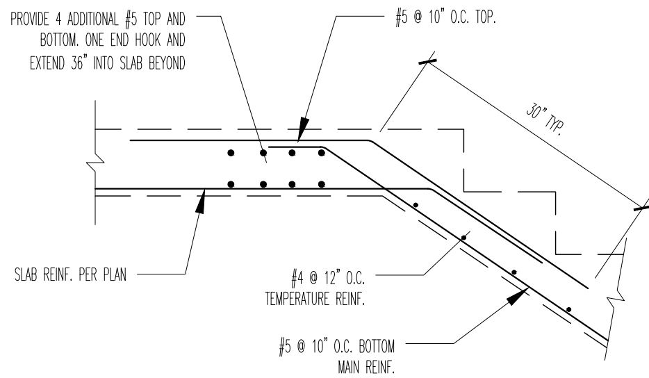
2 STAIR DETAIL SLAB LANDING SCALE 3/4" = 1'-0"
