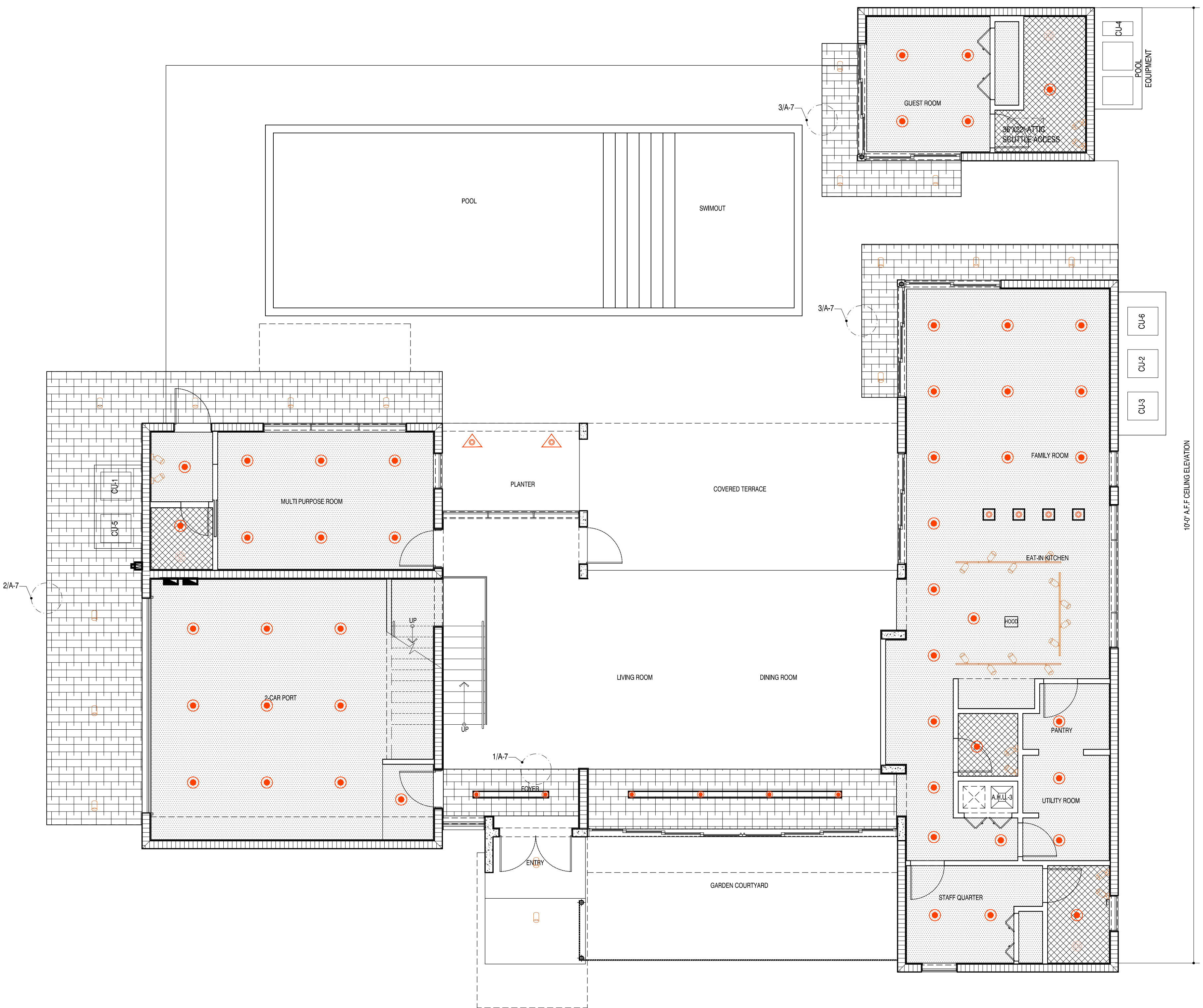
1st LEVEL REFLECTING CEILING PLAN SCALE: 3/16" = 1'-0"
